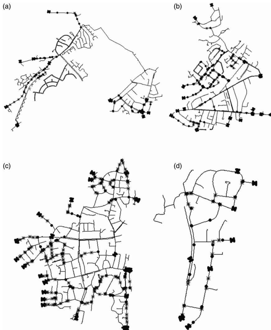
Figure 7 | Dead-end-like behaviour (black dots) caused by DMAs: (a) DMA 14, (b) DMA 5, (c) DMA 6, (d) DMA 15.
