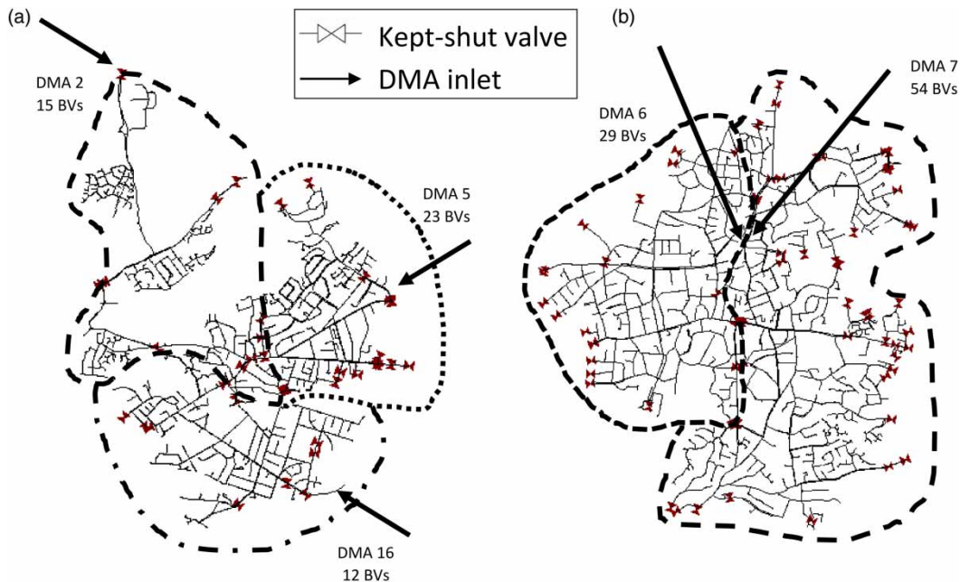
Figure 1 | Examples of DMA topology showing the spatial distribution of boundary valves (BVs) in the selected case study: (a) DMAs 2, 5 and 16, (b) DMAs 6 and 7.
