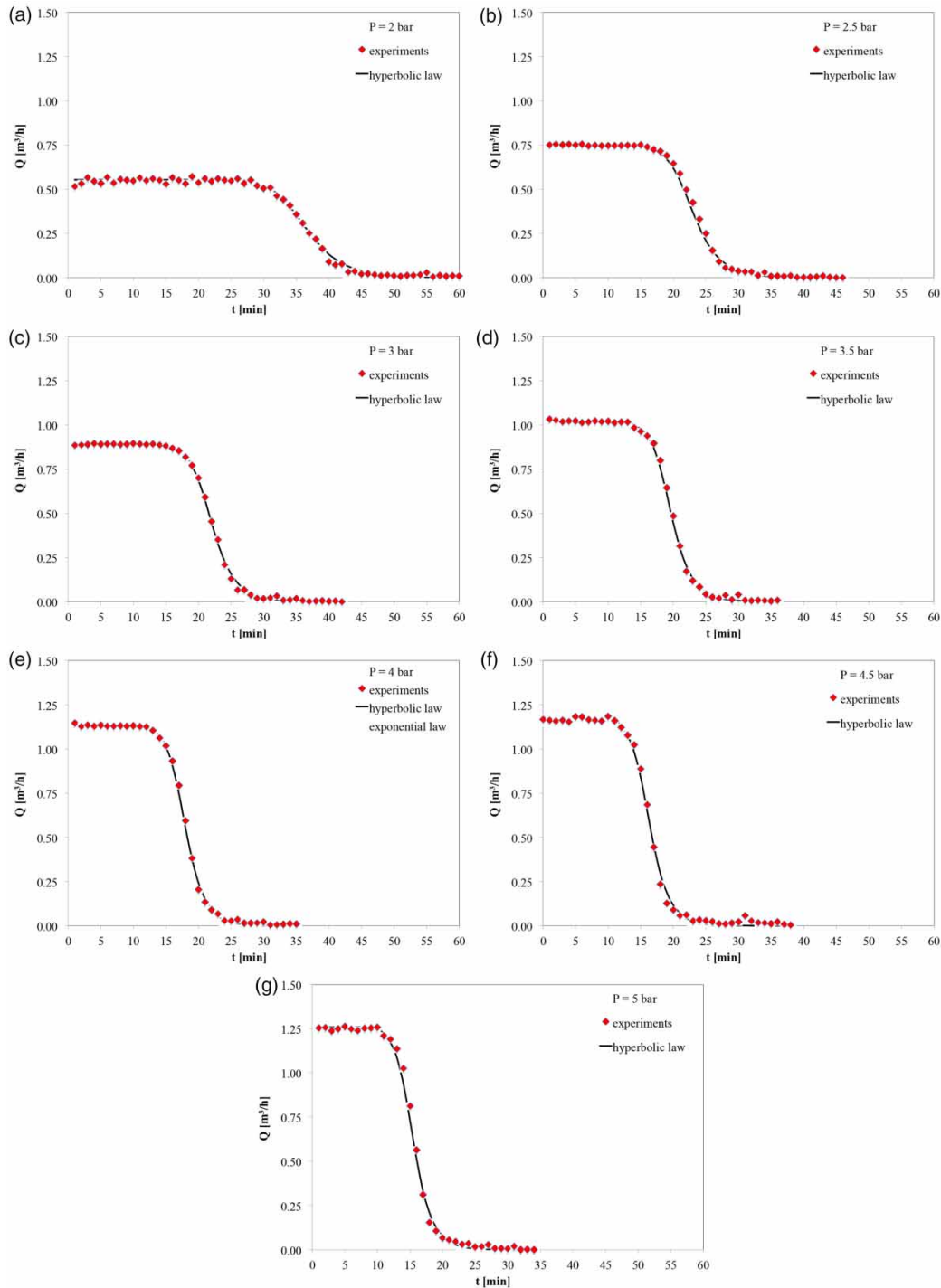
Figure 5 | TC3. Flow rate during the tank filling process, considering a constant value of a_n . Symbols: experiments; bold line: hyperbolic law. (a) Pressure 2 bar; (b) pressure 2.5 bar; (c) pressure 3 bar; (d) pressure 3.5 bar; (e) pressure 4 bar; (f) pressure 4.5 bar; (g) pressure 5 bar.
