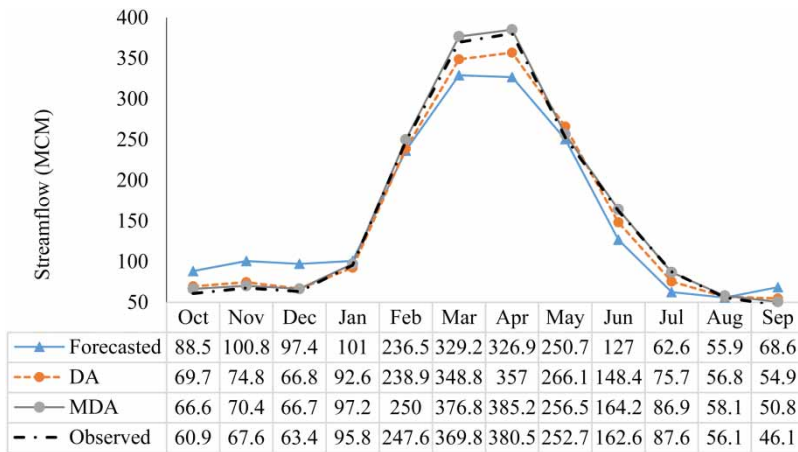
Figure 4 | Comparisons of monthly average streamflow values (MCM).
