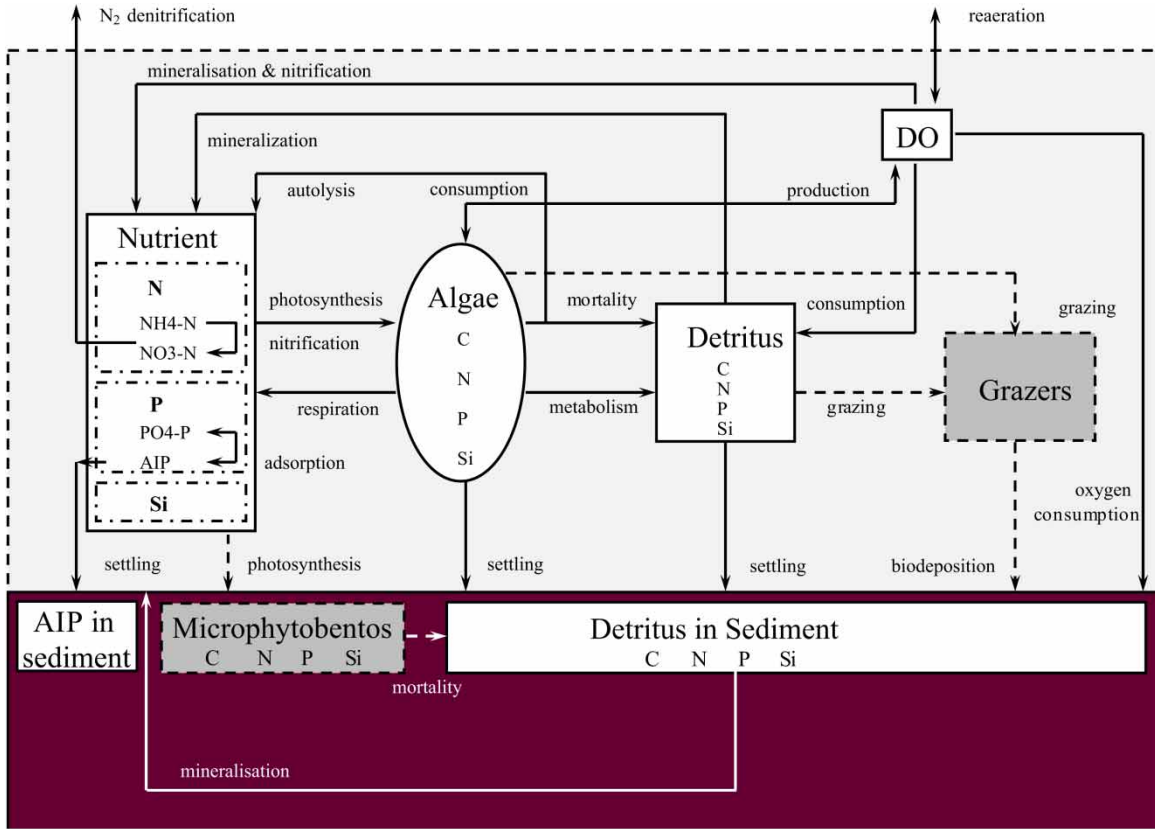
Figure 1 | State variables and processes in the GEM. State variables in grey and processes indicated by dashed lines have not been included in the North Sea modelling applications. AIP is adsorbed inorganic phosphorus. Source: Los et al. (2008).
