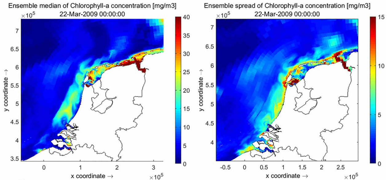
Figure 7 | Ensemble median prediction (left) and corresponding ensemble spread (right) of Chlorophyll-a concentration along the Dutch coast during the peak spring algal bloom in 2009.
