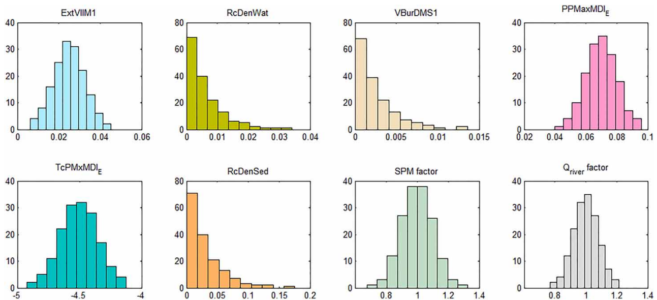
Figure 5 | Sample distribution of the selected significant parameters from LHS, n = 160 .
