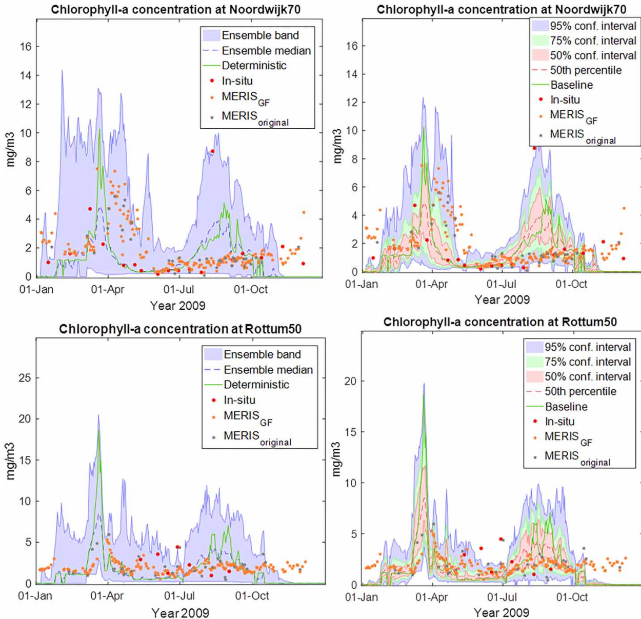
Figure 6 | Ensemble band (left) and confidence intervals (right) with the measurements at station Noordwijk 70 and Rottum 50, year 2009.
