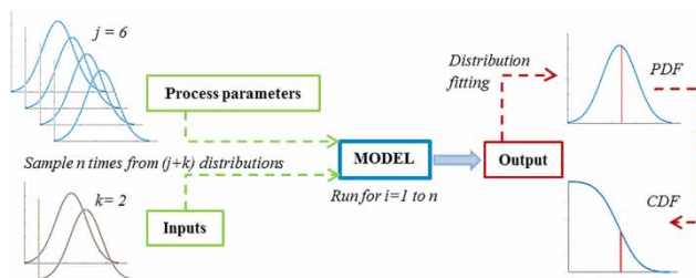
Figure 4 | Schematization of the ensemble forecasting methodology. PDF is probability density function and CDF is cumulative distribution function.
