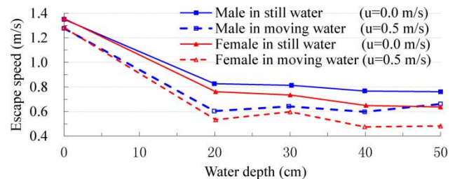
Figure 2 | Empirical curves related to the water depths and corresponding escape speeds for adults in floodwaters (from Ishigaki et al. 2008).
