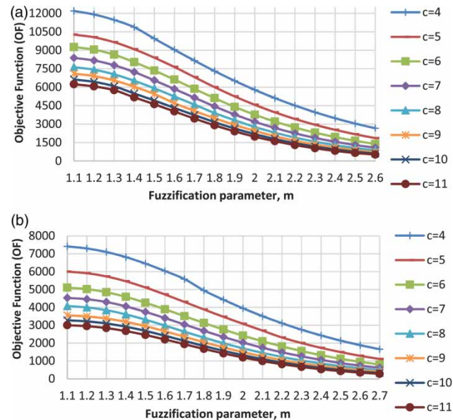
Figure 9 | Variation of objective function ( OF ) value for different m and c : (a) fuzzy clustering scenario 1 and (b) fuzzy clustering scenario 4.
