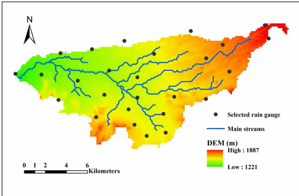
Figure 1 | DEM and selected rain gauges (cell size is 150 m).
