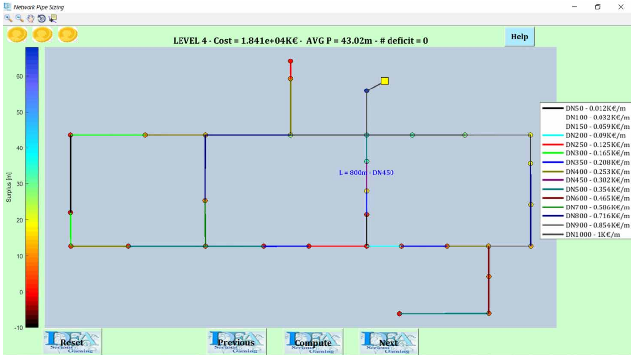
Figure 7 | Optimal solution screenshot of the fourth level of the NPS game for WDN sizing.
