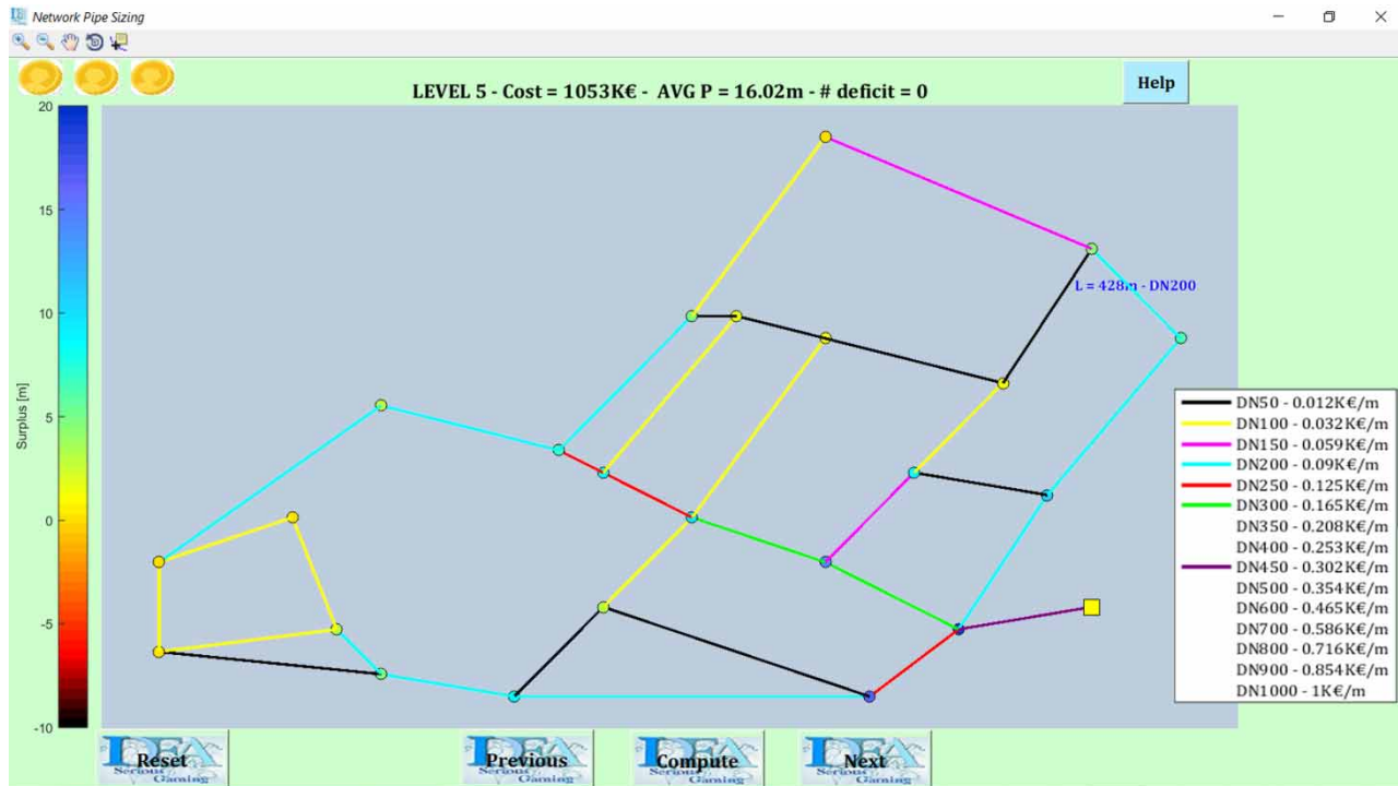
Figure 10 | Optimal solution screenshot of the fifth level of the NPS game for WDN sizing.
