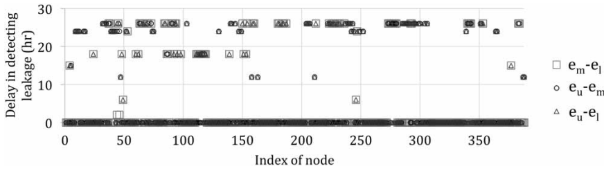
Figure 12 | The delay between the time of detection for Scenario 1 leakages when an ensemble of ten sensors is used. The error threshold is modeled at discrete values of 0.35, 0.70, and 1.05 psi. The sensor configuration is presented in Figure 11, respectively.
