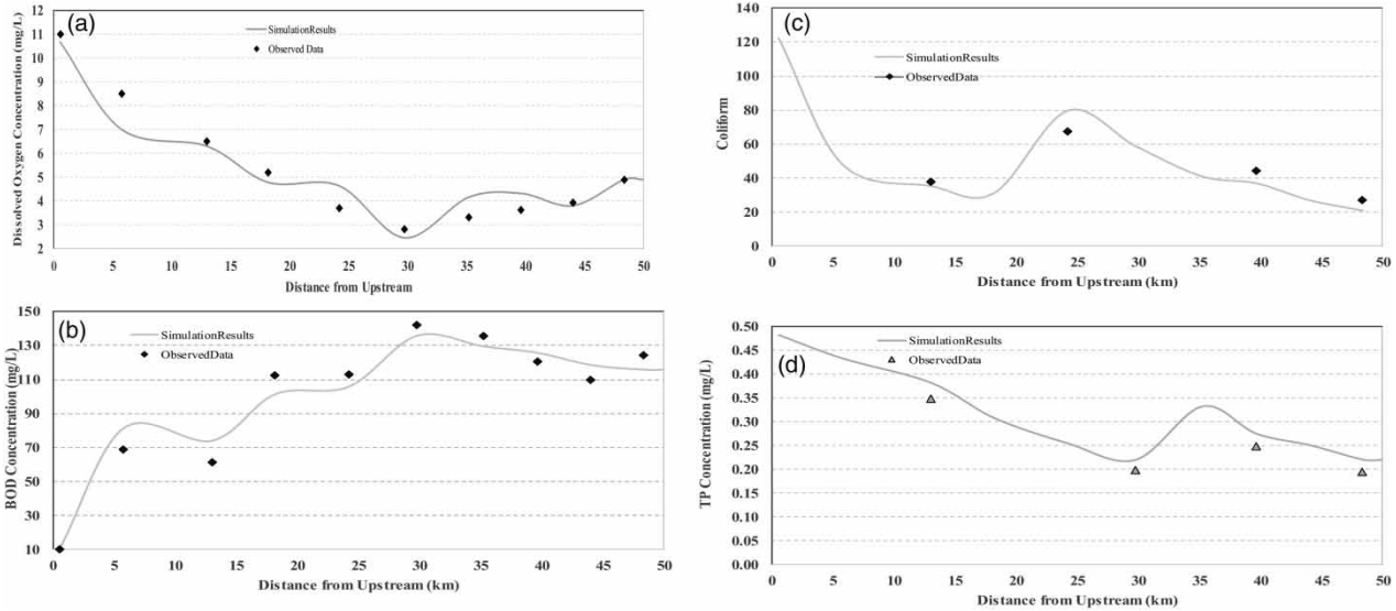
Figure 3 | The comparison results between observed data and QUAL2Kw model results in Gheslugh River: (a) dissolved oxygen, (b) BOD, (c) Coliform, and (d) total phosphorus (TP).
