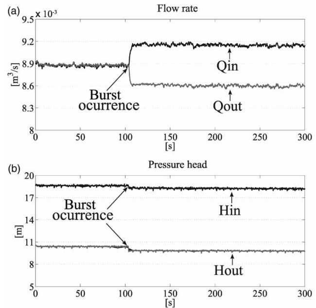
Figure 4 | Flow rate and pressure head at the ends of the pipeline (Experiment 1).
