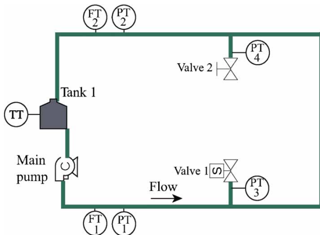
Figure 2 | Pipeline prototype diagram.
