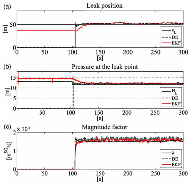
Figure 5 | Burst values and their estimations in Experiment 1.
