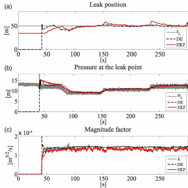
Figure 8 | Burst values and their estimations in Experiment 2.
