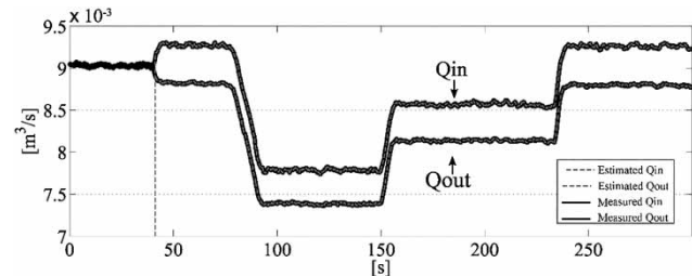
Figure 9 | Flow measures and their estimations in Experiment 2.
