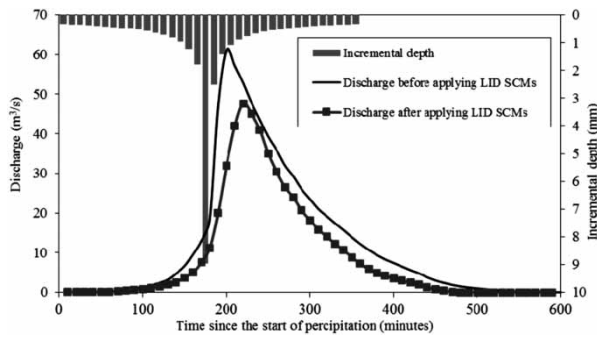
Figure 8 | Outflow hydrograph before and after the application of LID SCMs.
