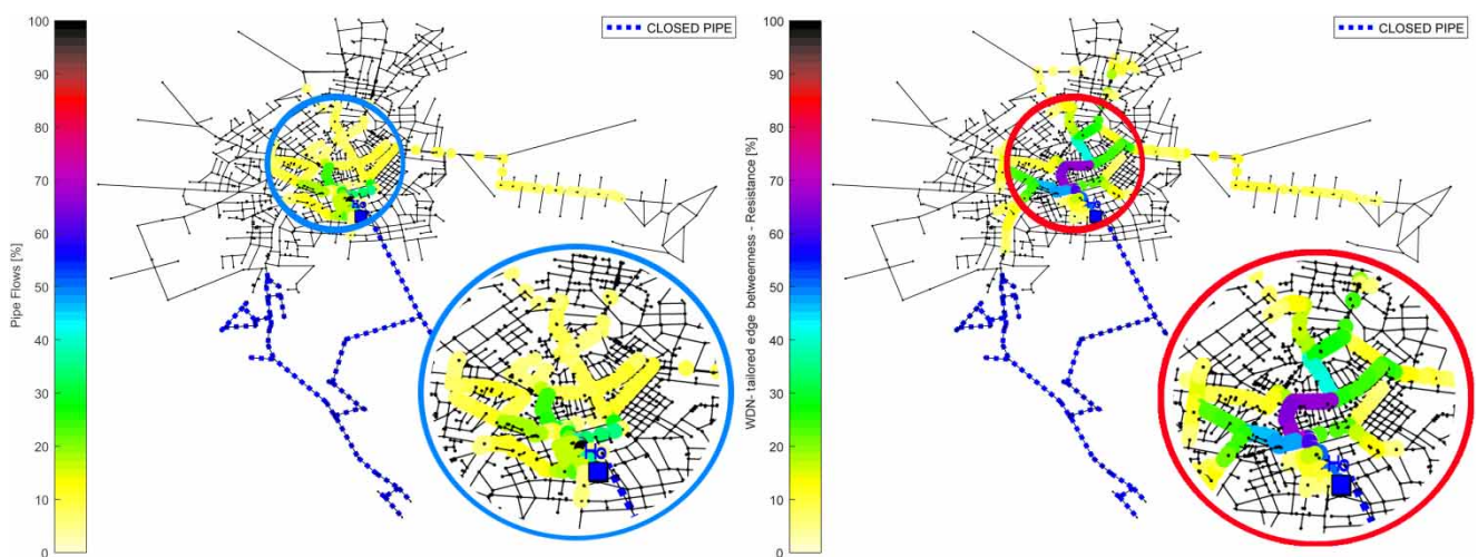
Figure 5 | Pipe with flow rates in the highest 5% values (left) and pipes with the highest 5% values of the WDN-tailored edge betweenness (right) for the Apulia 4 network. Spearman correlation index is equal to 0.66.
