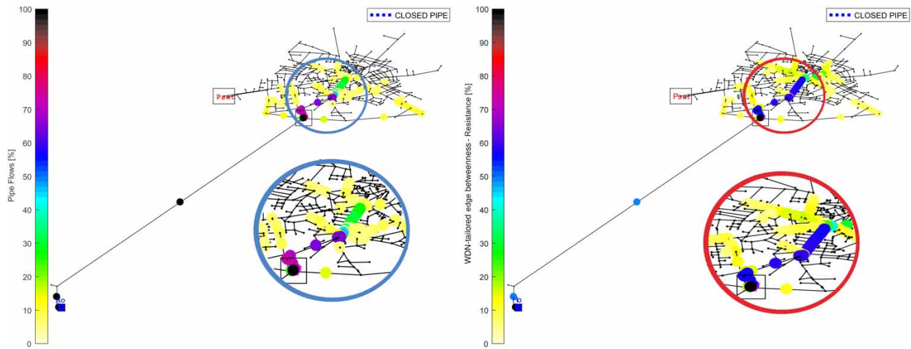
Figure 2 | Pipe with flow rates in the highest 5% values (left) and pipes with the highest 5% values of the WDN-tailored edge betweenness (right) for Apulia 1 network. Spearman correlation index is equal to 0.64.
