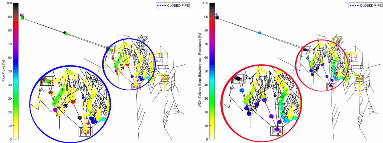
Figure 7 | Pipe with flow rates in the highest 5% values (left) and pipes with the highest 5% values of the WDN-tailored edge betweenness (right) for the Apulia 6 network. Spearman correlation index is equal to 0.54.
