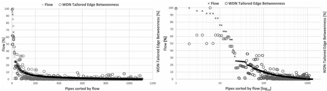
Figure 8 | Comparison between the pipe flows and the tailored edge betweenness.
