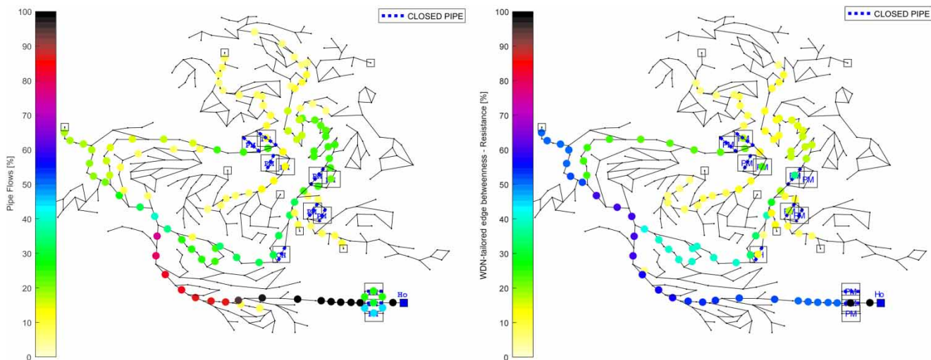
Figure 1 | Pipe with flow rates in the highest 5% values (left) and pipes with the highest 5% values of the WDN-tailored edge betweenness (right) for BBLAWN network. Spearman correlation index is equal to 0.74.
