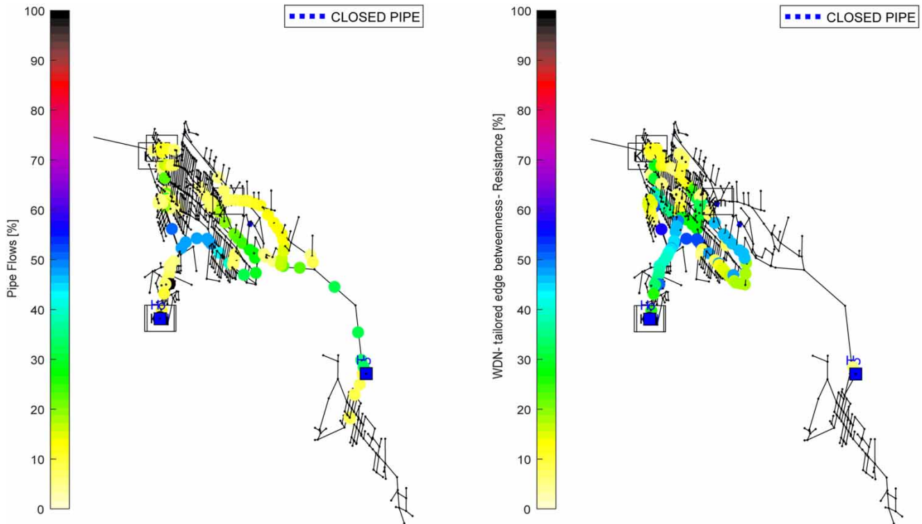
Figure 4 | Pipe with flow rates in the highest 5% values (left) and pipes with the highest 5% values of the WDN-tailored edge betweenness (right) for the Apulia 3 network. Spearman correlation index is equal to 0.54.
