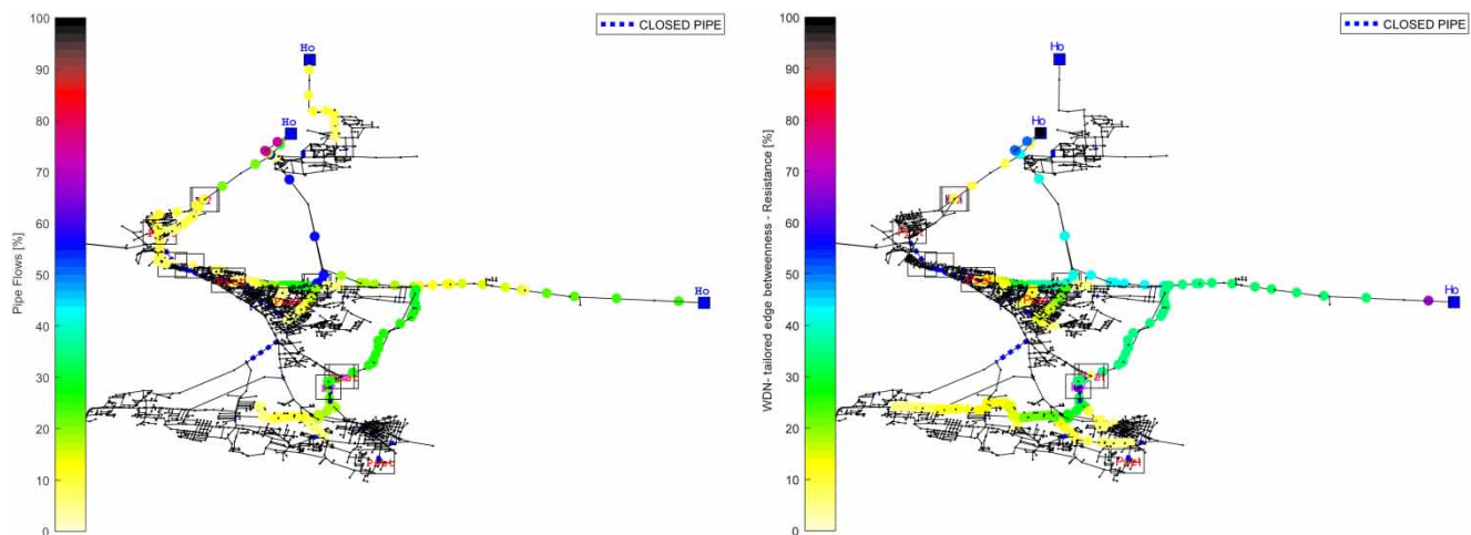
Figure 3 | Pipe with flow rates in the highest 5% values (left) and pipes with the highest 5% values of the WDN-tailored edge betweenness (right) for the Apulia 2 network. Spearman correlation index is equal to 0.60.
