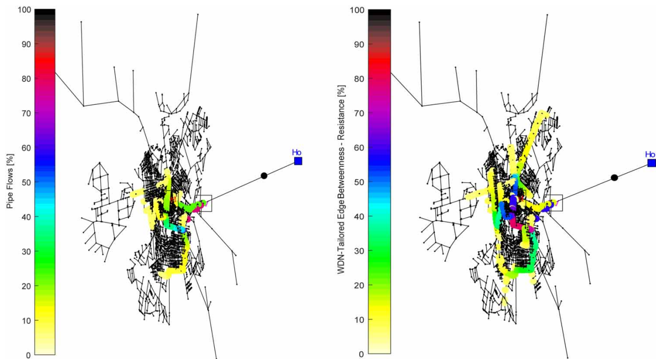
Figure 6 | Pipe with flow rates in the highest 5% values (left) and pipes with the highest 5% values of the WDN-tailored edge betweenness (right) for the Apulia 5 network. Spearman correlation index is equal to 0.62.
