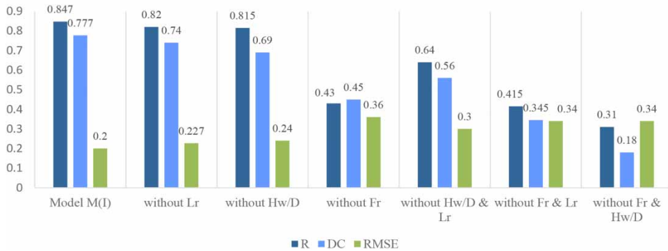
Figure 7 | Relative significance of each of the input parameters of the best model (M (I)).
