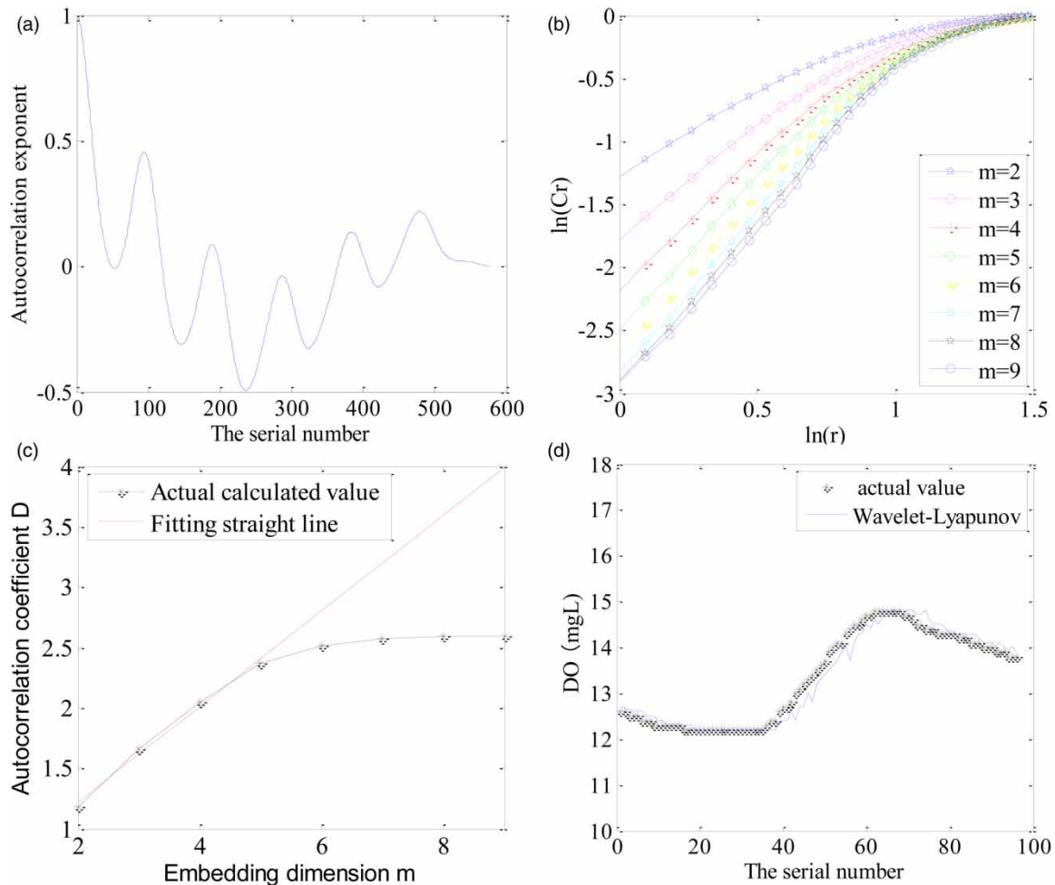
Figure 10 | Chaos characteristics of high-frequency DO time series: (a) variation of autocorrelation, (b) \ln C(r) versus \ln(r) , (c) relationship between correlation exponent and embedding dimension, and (d) forecast results.
