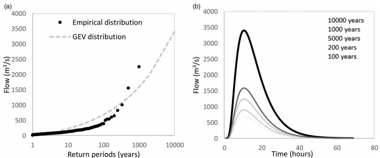
Figure 4 | Annual maximum flows (a) and flood hydrographs for different return periods (b) at the Zavoj reservoir (Pirot water resources system).
