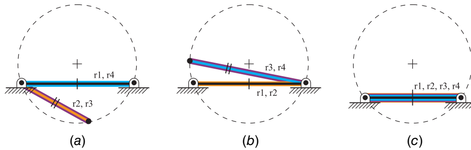
Fig. 11 Class 3 change-point mechanisms in their conformed positions. Hatch marks indicate equal link lengths: (a) CP2X where r_2 = r_3 and r_1 = r_4 , (b) CP2X where r_1 = r_2 and r_3 = r_4 , and (c) CP3X where all links lie in the same position.
