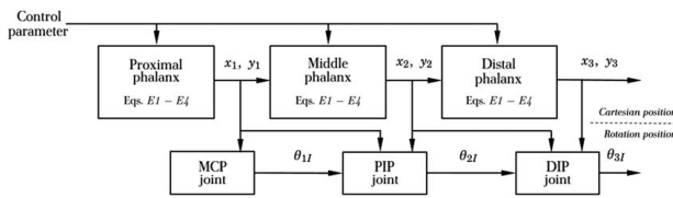
Fig. 2 Numerical framework for calculating the joint angles of a finger (modified from Ref. [9])
