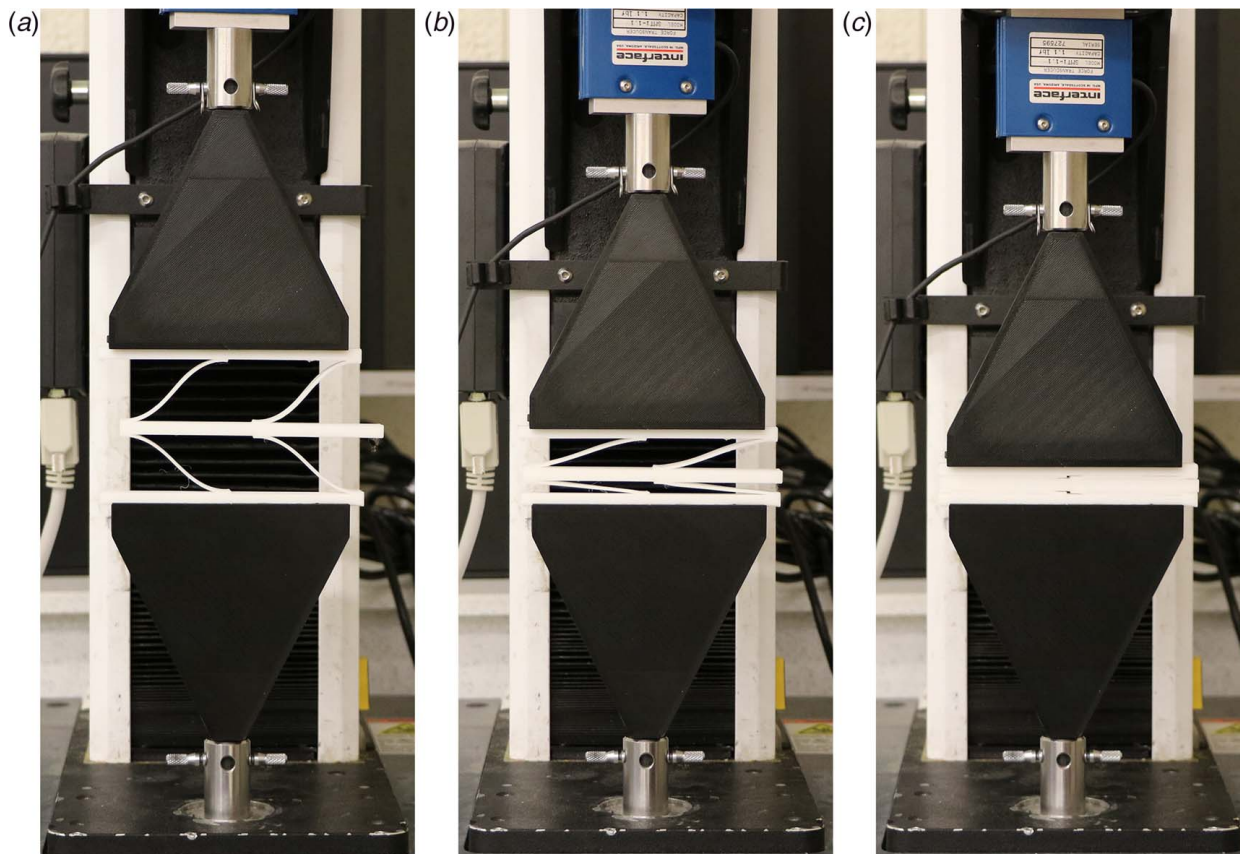
Fig. 11 Experimental setup and compression testing of the DESCs: (a) experimental test setup with DESC fully expanded, (b) compression test with the DESC partially compressed, and (c) compression test with the DESC fully compressed
