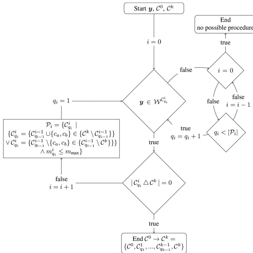
Fig. 3 Algorithm for configuration determination
