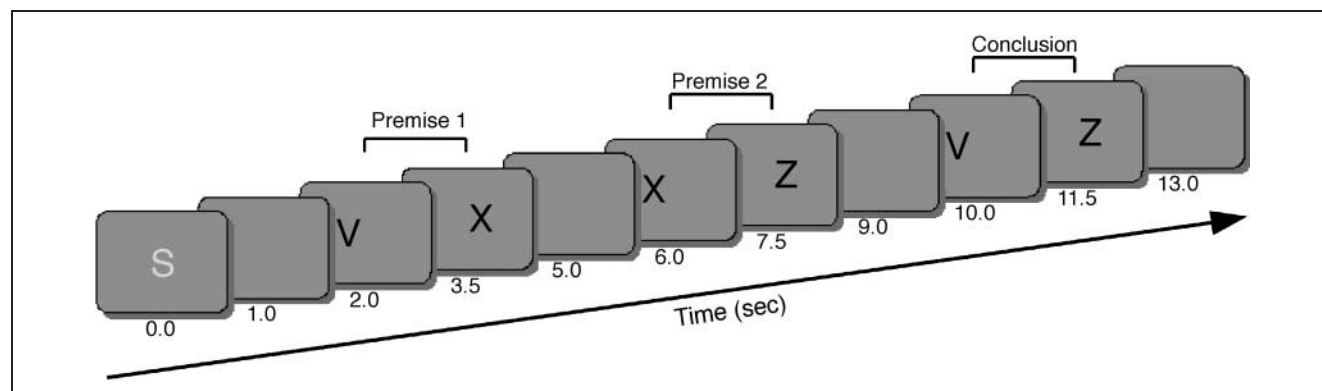
Figure 1. Sequence of a reasoning problem. Prior to each problem, an “S” (“Schließen” in German) or an “E” (“Erinnern” in German) was presented for 1 sec. The spatial relation between the two letters of each premise or conclusion was coded by placing it right or left from the midpoint of the screen. Each trial began with presentation of the first letter for 1500 msec, followed by the second letter for 1500 msec, and a pause for 1000 (first premise), making a total of 4 sec. The period for the second premise and the conclusion or maintenance was the same as during the first premise.
