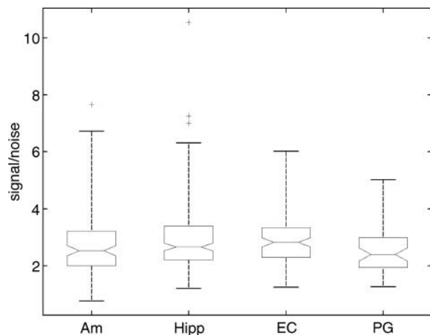
Figure S1. Signal-to-noise ratios in indifferent brain areas. Boxplot of the signal-to-noise ratios in different brain areas. Horizontal middle lines represent medians of distributions of signal-to-noise ratios.
