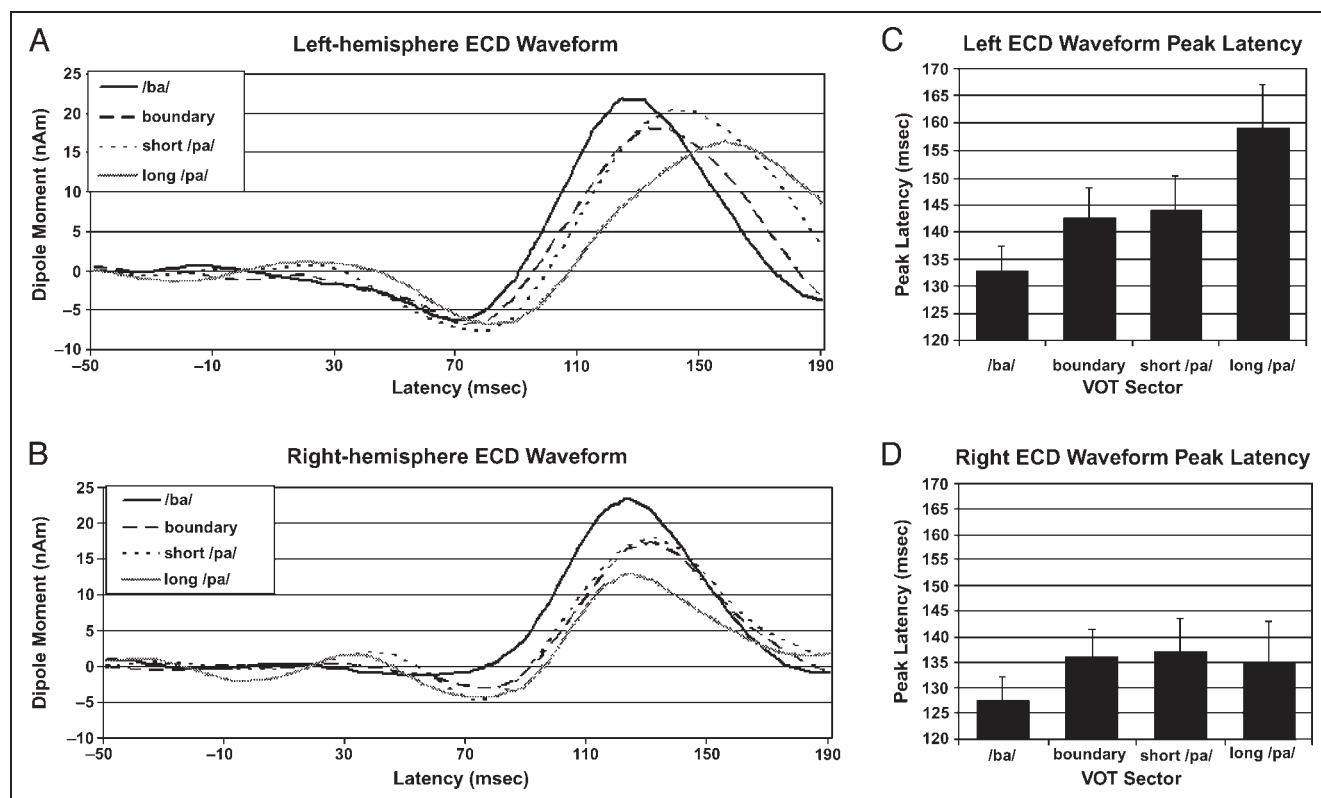
Figure 3. The waveforms derived from the equivalent current dipole (ECD) model averaged across participants for each VOT continuum sector for the left (A) and right (B) hemispheres. Waveform peak latency is dependent on VOT in the left (C) but not the right (D) hemisphere.
