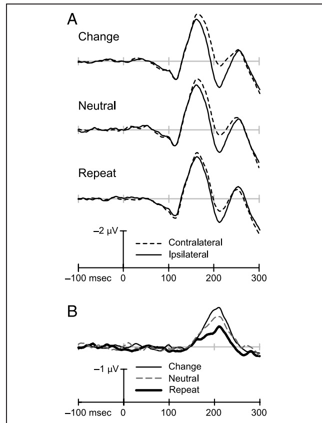
Figure 2. Grand averaged ERP waveforms time-locked to S2 in repeat, neutral, and change conditions, recorded at lateral occipital electrode sites (PO7, PO8). The time scales are referenced to the onset of S2 at 0 msec. Negative voltage is plotted upward. (A) ERPs recorded contralateral and ipsilateral to the target side, collapsed over left-target and right-target displays. (B) ERP difference waves created by subtracting the ipsilateral-to-target waveform from the contralateral-to-target waveform.
