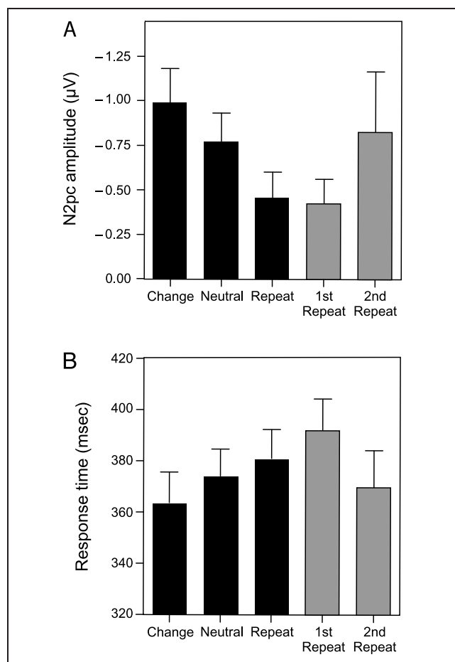
Figure 3. Mean response times and N2pc amplitudes for S2 target displays. Black bars show results from repeat, neutral, and change conditions, and gray bars show results from the first and second repeated target displays separately. Standard error bars are shown. (A) N2pc amplitudes. (B) Response times.
