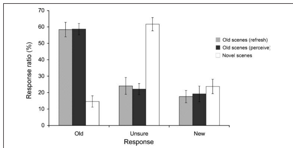
Figure 3. Scene recognition.
