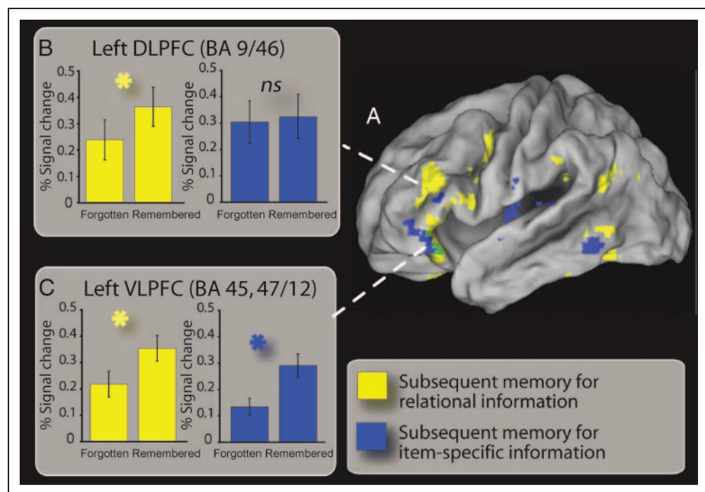
Figure 2. DLPFC activity specifically correlates with subsequent memory for relational information. (A) At upper right, a cortical surface rendering shows regions (colored in yellow) for which activity was increased during relational encoding ( interact ) trials for which the relational information was remembered with high confidence compared with relational trials for which this information was forgotten. Also depicted are regions (colored in blue) for which activity was increased on item-specific encoding ( separate ) trials for which the location of both items was subsequently remembered with high confidence compared with trials for which the location of the items was subsequently forgotten. Regions colored in green exhibited suprathreshold responses in both contrasts.
