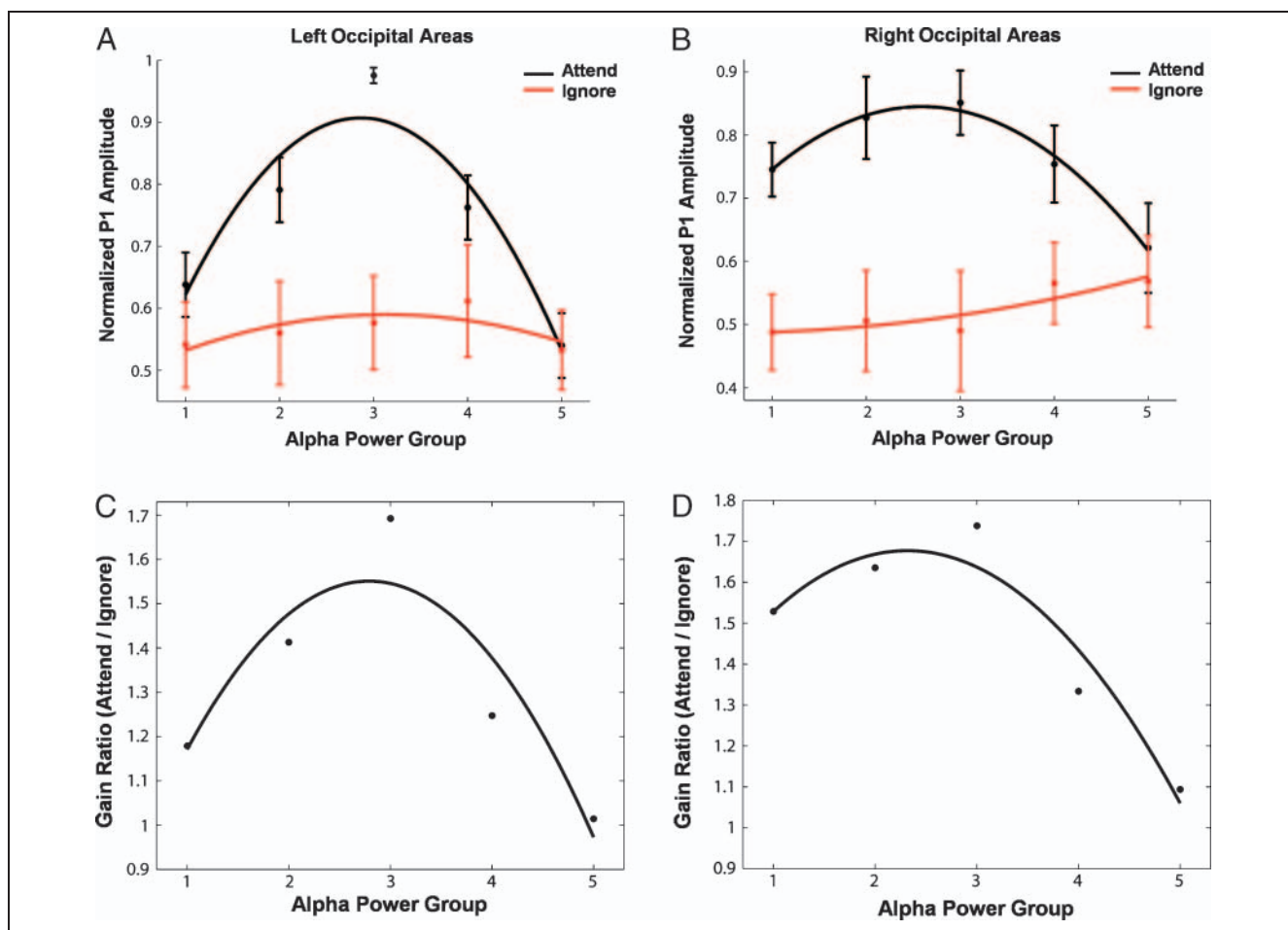
Figure 8. Gain ratio as a function of prestimulus alpha. P1 amplitude as a function of prestimulus alpha power is plotted for both attend and ignore conditions in (A) and (B). The ratios between the two curves are shown in (C) and (D). Maximum gain is achieved for intermediate levels of prestimulus alpha activity.
