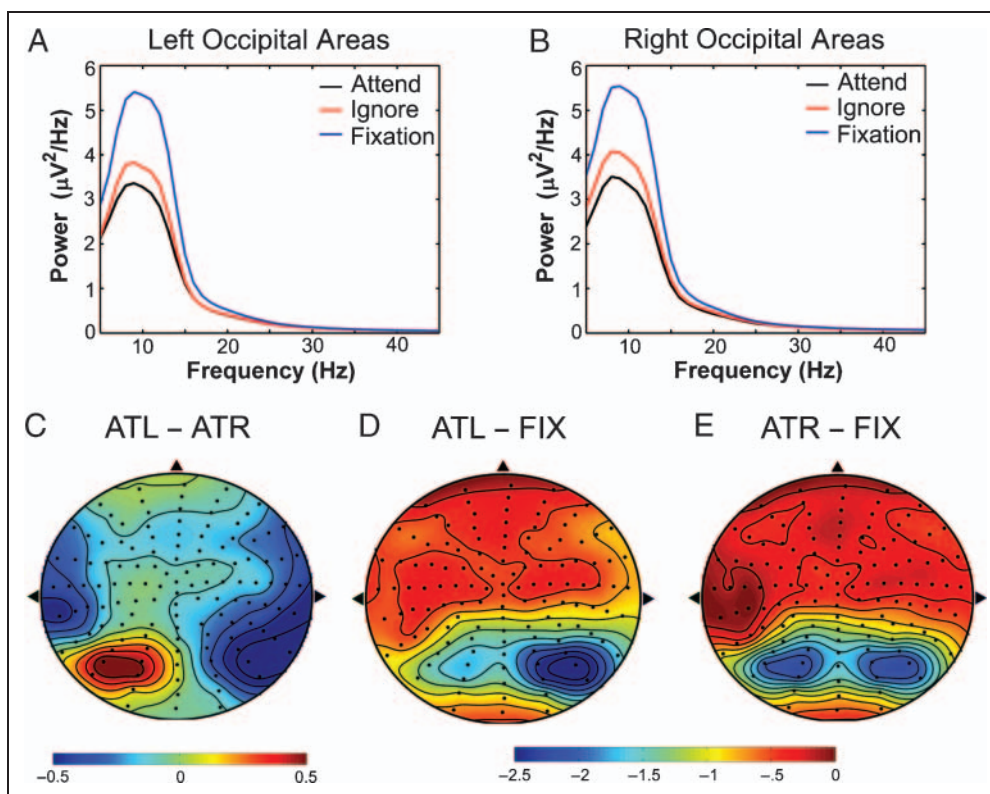
Figure 3. Attentional modulation of alpha band activity. Power spectra: (A) left parieto-occipital and (B) right parieto-occipital areas. Black: attend contralateral visual field; red: ignore contralateral visual field (attend ipsilateral visual field); blue: relaxed fixation. (C–E) Scalp topography of alpha band power differences: (C) attend-left (ATL) minus attend-right (ATR), (D) attend-left minus relaxed fixation (FIX), (E) attend-right minus relaxed fixation.
