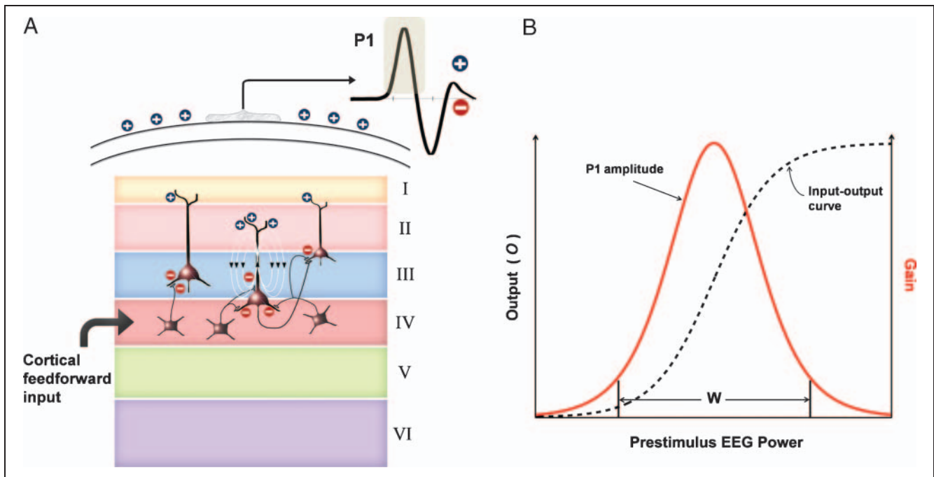
Figure 5. Model reformulation in terms of EEG variables. (A) Neural genesis of visually evoked P1. Feedforward activation of layer 4 stellate cells excites the basal dendrites of the superficial layer pyramidal cells, leading to an extracellular sink near layer 4 and an extracellular source, composed mainly of passive return current, near the cortical surface. The latter is sensed by the scalp electrode as a positive-going ERP component. (B) Reformulated model in which prestimulus EEG power in alpha band is equated with level of background synaptic activity and magnitude of P1 with intensity of stimulus-evoked response. This model predicts that the P1 amplitude is an inverted-U function of prestimulus alpha power with the variable W defining a range of effective operation.
