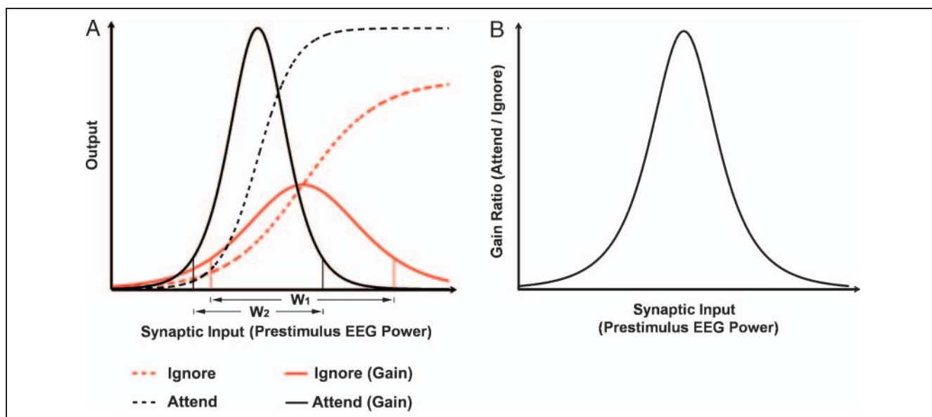
Figure 7. Schematic illustration of attentional modulation mechanisms of ongoing activity. (A) Attention shifts the sigmoidal curve in Figures 4 and 5 leftward and increases its overall slope (global gain). (B) The ratio of the gain curves in (A) for attend and ignore conditions is again an inverted-U function.
