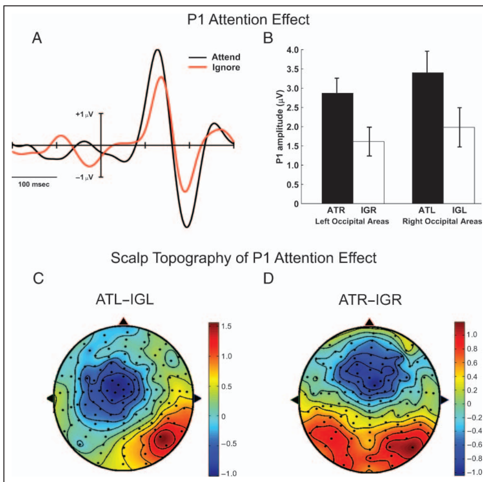
Figure 2. ERP analysis. (A) Typical waveforms of visual ERP over the parieto-occipital region contralateral to the visual field of stimulation. Attentional enhancement of P1 and N1 components is apparent. (B) P1 amplitudes to contralateral stimulation averaged over channels and subjects. (C–D) Scalp distribution of attentional enhancement of posterior P1 (shaded red) and fronto-central N1 (shaded blue) at 120 msec after presentation of the standard stimulus. ATL = attend-left; IGL = ignore-left; ATR = attend-right; IGR = ignore-right.
