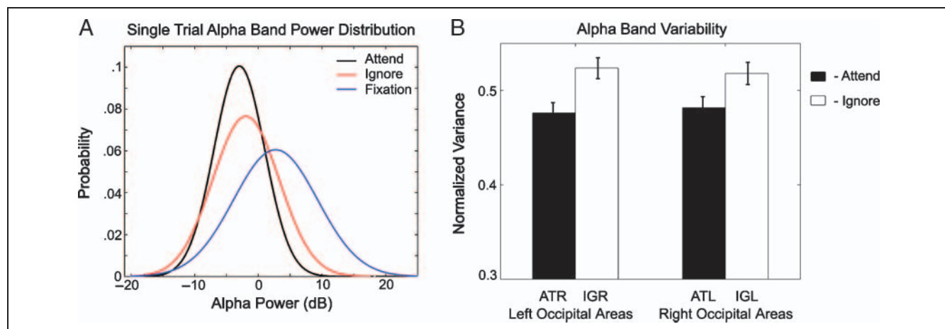
Figure 9. Distribution of alpha power. (A) Distributions of log-transformed single-trial alpha power for attend, ignore, and fixation conditions over left parieto-occipital areas from a representative subject. Variance of the single-trial alpha power distribution is compared over subjects between attend and ignore conditions in (B) where a reduction in variance is taken as evidence of decreased trial-to-trial alpha power variability.
