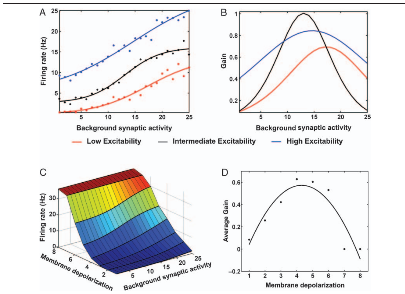
Figure 10. Computational study of relation between excitability and gain. (A) Firing rate over a 200-msec interval as function of background synaptic activity for three levels of mean membrane depolarization (blue: high excitability; black: intermediate excitability; and red: lower excitability). (B) Derivative of the sigmoidal curves in (A) showing nonlinear relationship between gain and background synaptic activity. (C) Firing rate as a function of mean membrane depolarization levels and variance of background synaptic activity. (D) Average gain, which corresponds to average stimulus-evoked response, for increasing levels of membrane depolarization.
