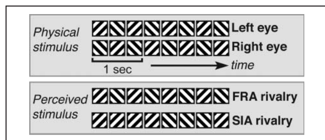
Figure 1. IOS rivalry stimuli and percepts. Orthogonal gratings are exchanged between the eyes three times per second. These stimuli give rise to two types of visual percepts: fast, regular alternations in perceived orientation that are time-locked to the stimulus exchanges (FRA rivalry) or slow, irregular orientation alternations that span multiple IOSs (SIA rivalry).
