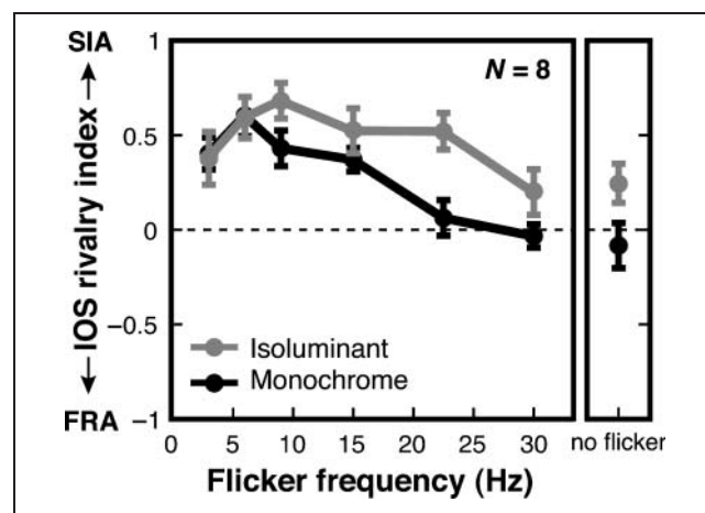
Figure 3. Results of Experiment 2. Isoluminance increases the amount of SIA rivalry in IOS rivalry. Monochrome (black–white) or isoluminant (red–green) gratings with different flicker frequencies were presented on a gray background. Subjects perceived more SIA rivalry for isoluminant gratings (gray line) than for monochrome gratings (black line). Error bars are SEM.
