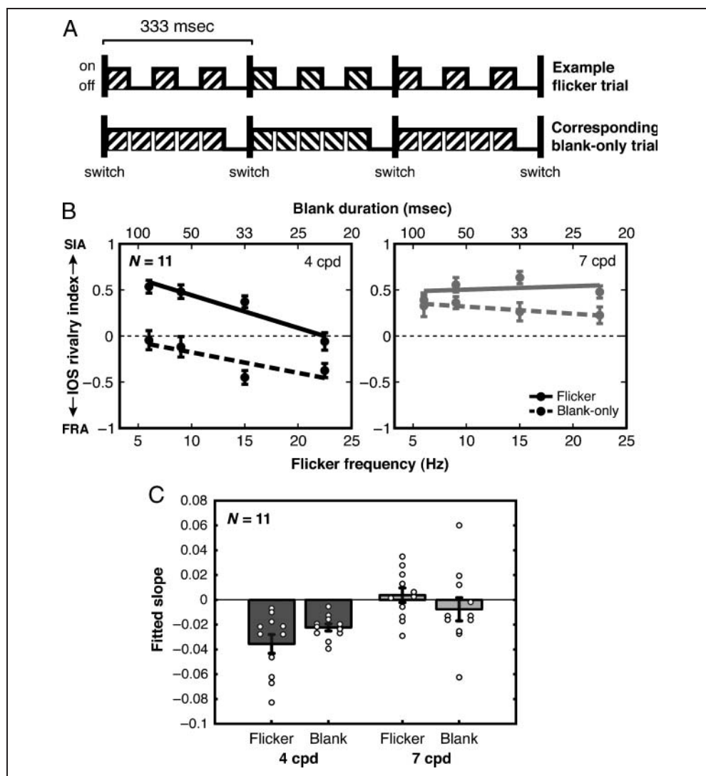
Figure 4. Stimulus design and results for Experiment 3. Short preswitch blanks promote FRA rivalry for low spatial frequency IOS rivalry gratings. (A) Two types of stimuli were constructed. The stimulus sequence is shown for only one of the eyes. Continuous-flicker stimuli flickered on and off with a 50% duty cycle in one of four flicker frequencies in different trials. For each flicker frequency, a corresponding blank-only stimulus was constructed in which gratings were always on except during a short blank period immediately preceding the IOS. The duration of this blank period was the same as the duration of the preswitch off period in the corresponding continuous-flicker condition. In the example shown here, the flicker frequency is 9 Hz, and the corresponding blank duration is 56 msec. (B) Two spatial frequencies and four flicker frequencies were tested for both the continuous-flicker (solid lines) and blank-only (dotted lines) conditions. For low spatial frequency stimuli (4 cpd, left, black lines), increases in flicker frequency and decreases in blank duration both resulted in increased FRA rivalry. High spatial frequency stimuli (7 cpd, right, gray lines) showed no effect of either flicker frequency or blank duration on the IOS rivalry index. (C) Linear functions were fit to individual subject data for each spatial frequency–flicker condition. Means of the fitted slopes for each condition are plotted as bars (dark = low spatial frequency; light = high spatial frequency). Error bars are SEM . Fitted slopes for individual subjects are shown as white circles.
