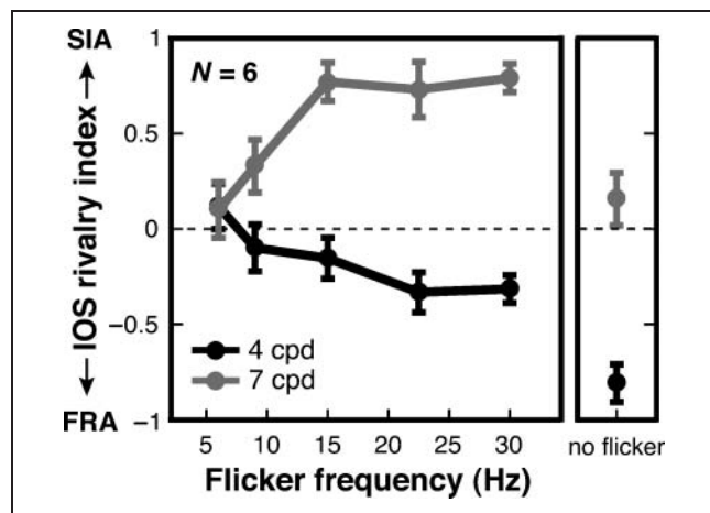
Figure 2. Results of Experiment 1. Spatio-temporal interaction in IOS rivalry. IOS rivalry gratings with high or low spatial frequencies and different on–off flicker frequencies were presented on a gray background. As flicker frequency increased, the predominance of SIA rivalry increased for high spatial frequency gratings (7 cpd, gray line) but decreased for low spatial frequency gratings (4 cpd, black line). Error bars are SEM.
