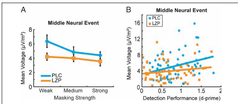
Figure 5. Effect of masking strength on the middle event for LZP and PLC. (A) For PLC increasing masking strength reduced the neural activity in a linear manner. (B) The scatter plot for the middle event shows a positive correlation between the size of the deflection and detection performance.
