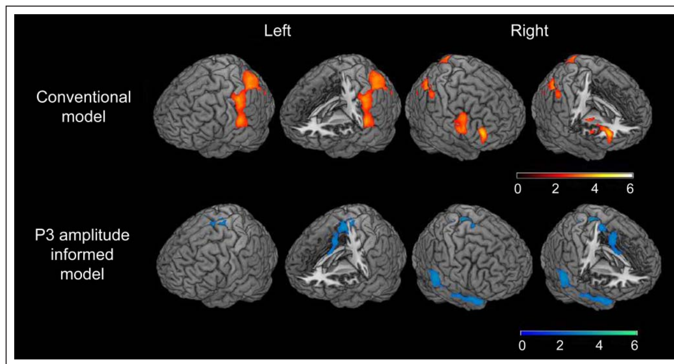
Figure 5. Nicotine effects on BOLD activation that covary with the nicotine effect on RT for the conventional and P3 informed models (second-level mixed-effects FLAME, n = 19 , cluster-corrected threshold Z = 2.3 , p = .05 ). There is a positive relationship between the change in RT and change in BOLD activation from the placebo condition to the nicotine condition in the conventional model (red scale), whereas there is a negative relationship (blue scale) for the P3 amplitude informed model.
