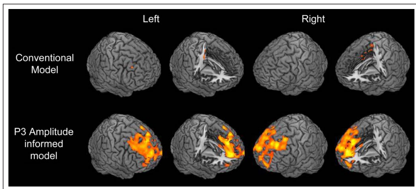
Figure 4. Nicotine effects (nicotine > placebo) on the BOLD response to target stimuli (target > baseline) for both the conventional and P3 amplitude informed models (second-level mixed-effects FLAME, n = 19 , cluster-corrected threshold Z = 2.3 , p = .05 ).
