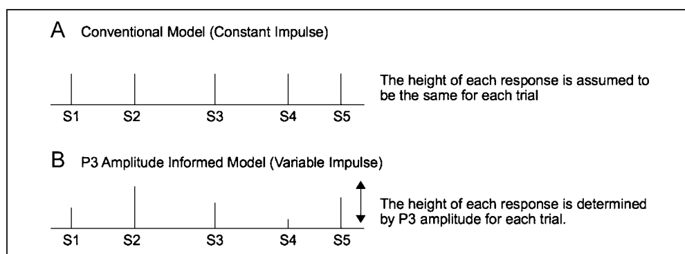
Figure 1. Summary of how the basis function is modified by including single-trial parameters in the GLM. (A) The conventional analysis where a constant impulse (same height and duration) is positioned at stimulus onset. (B) A variable impulse model where the height of the basis function is modified by single-trial P3 amplitude. When P3 amplitude was included in the model, this resulted in the height of the basis function being higher when P3 amplitude was larger. This reflects differences in the intensity of responses, as reflected in P3 amplitude. For both models, the input functions (onset time, event duration, and event intensity) were convolved with the gamma HRF, which blurs and delays the waveform to match the difference between the input function and the measured hemodynamic response.
