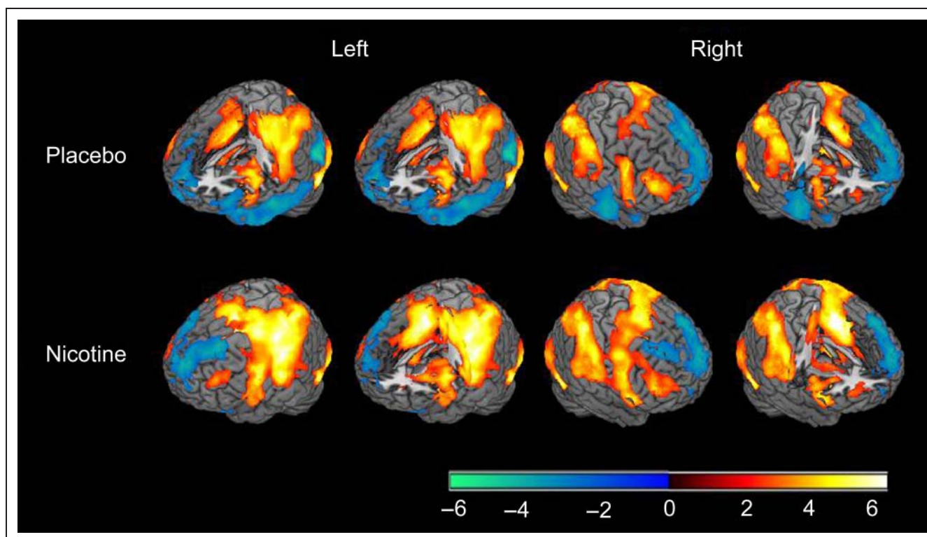
Figure 3. BOLD activation (target > baseline, red) and deactivation (target < baseline, blue) for the conventional analysis (second-level mixed-effects FLAME, n = 19 , cluster-corrected threshold Z = 2.3, p = .05 ) for the placebo and nicotine conditions.
