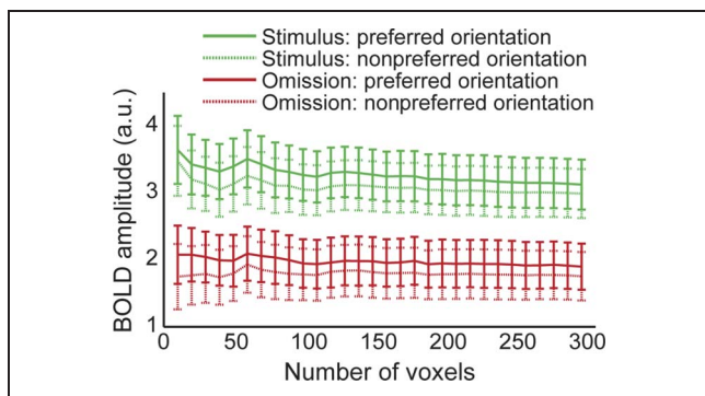
Figure 3. Orientation-specific BOLD signal in V1 for different numbers of selected voxels. Stimuli (green) and omissions (red) evoke stronger activity in voxels that prefer the currently presented or expected orientation (solid lines) than in voxels that prefer the orthogonal orientation (dashed lines) over a wide range of selected voxels. Error bars indicate SEM .
