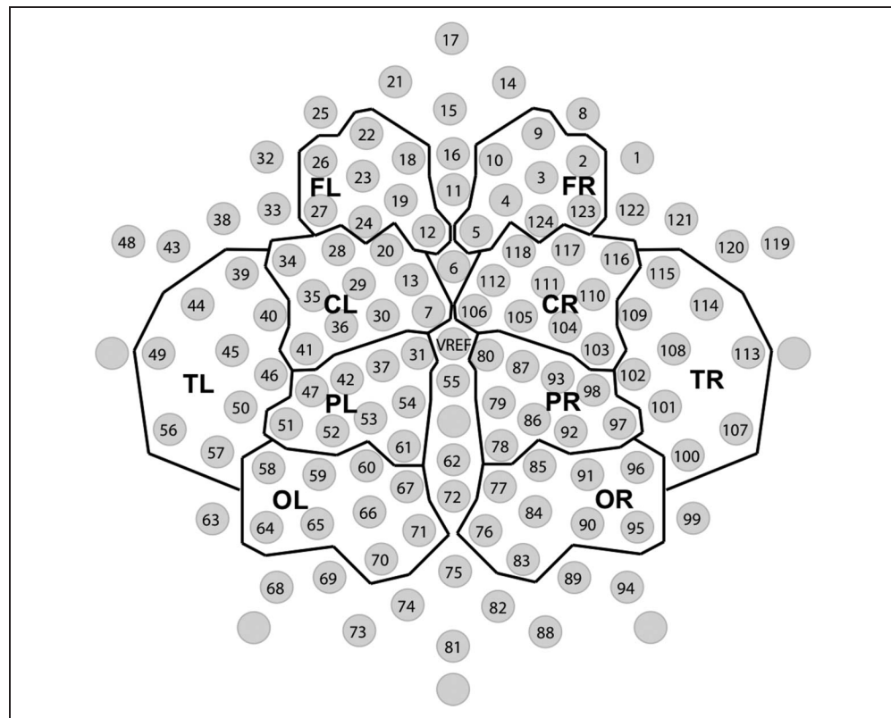
Figure 1. Electrode groupings (see Methods for details). Ninety of 124 electrodes were divided into five regions (frontal, central, parietal, occipital, and temporal) for each hemisphere. Each region contained between 16 and 20 electrodes that were averaged to represent EEG responses from that scalp region. The remaining channels around the perimeter of the net were excluded from analysis to avoid artifacts resulting from muscle activity in the face and neck, and channels along the midline were removed to allow for comparison between hemispheres.
