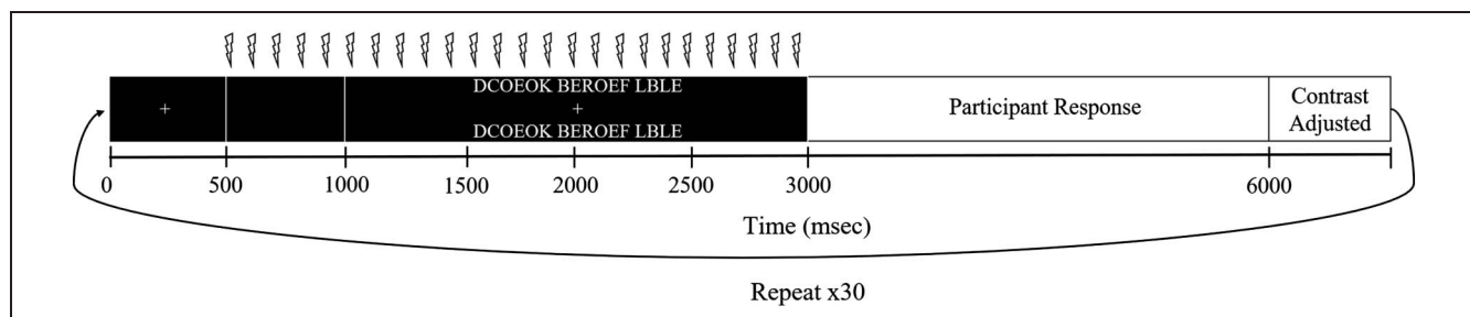
Figure 3. Illustrating the timing of events on an average visual discrimination threshold trial. Repetitive TMS (represented by lightning bolts) start 500 msec before the onset of the target visual stimuli. Repetitive TMS and target stimuli offsets occurred concurrently.
