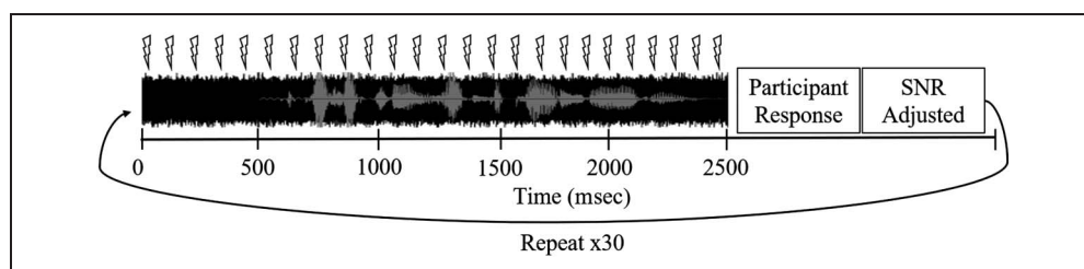
Figure 1. Illustrating the timing of events on an average SRT trial. Repetitive TMS and noise (represented by lightning bolts and black broadband waveform, respectively) start 500 msec before the onset of the target sentence (represented by the gray waveform). Repetitive TMS, noise, and target sentence offsets all occurred concurrently.
