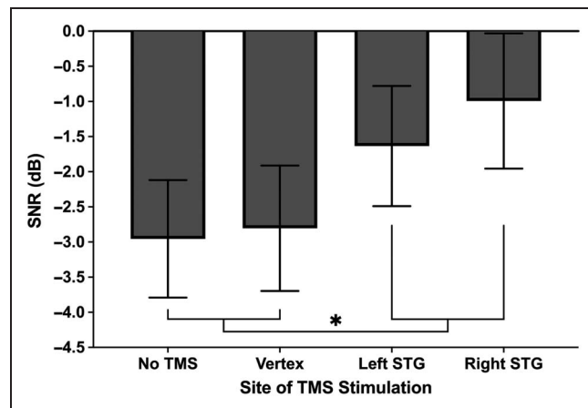
Figure 2. Depicting the average SNR level at the point of a reversal across the four sites of TMS stimulation. Error bars represent 95% confidence intervals. * p < .01 .
