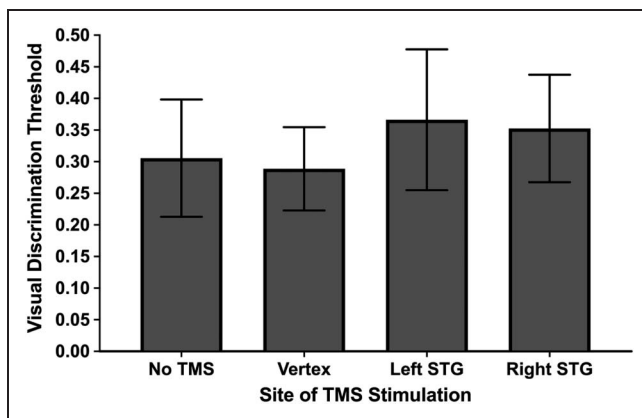
Figure 4. Depicting the average contrast level (RGB) at the point of a reversal across the four sites of TMS stimulation. Error bars represent 95% confidence intervals.
