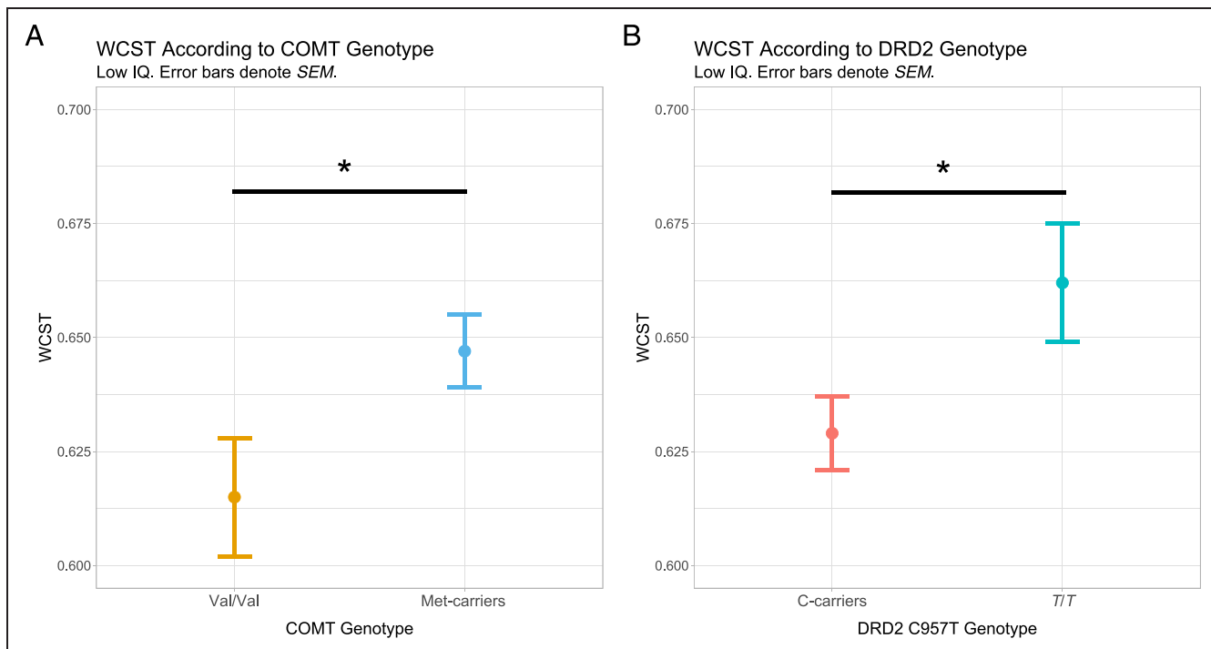
Figure 1. WCST accuracy rate according to (A) COMT genotype and (B) DRD2 C957T genotype, in low IQ participants, controlling for age and gender. *p < .05 .
