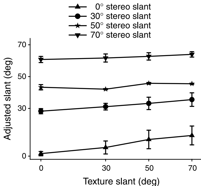
Figure 12. The average judged slants for all of the different combinations of texture- and stereo-defined slant in Experiment 3.
