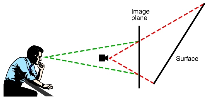
Figure 4. A schematic diagram of an image of a surface that is viewed with a different visual angle from the one at which it was photographed or rendered. The camera angle in this example is represented by dashed red lines, and the viewing angle is represented by dashed green lines.
