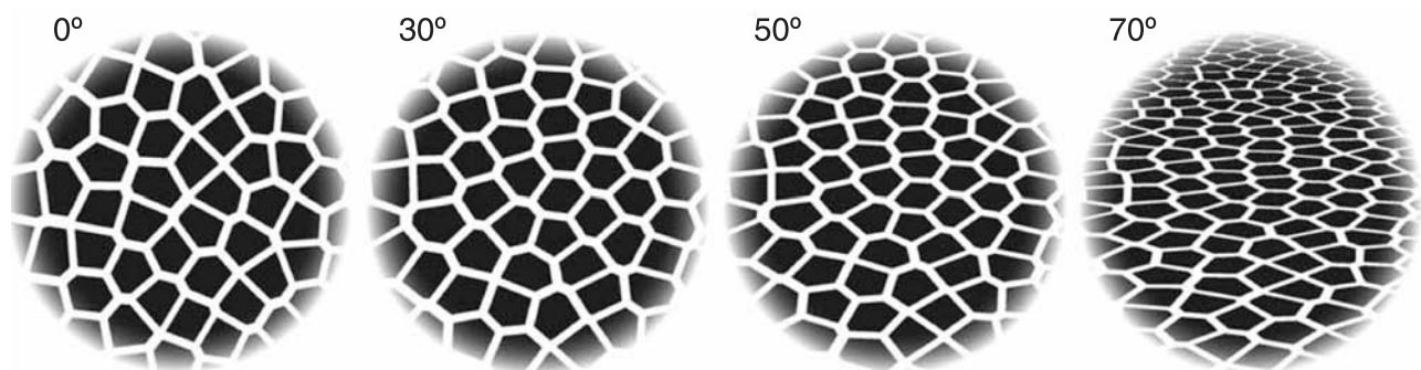
Figure 3. Some stimuli used by Knill and Saunders (2003) in a slant discrimination study.
