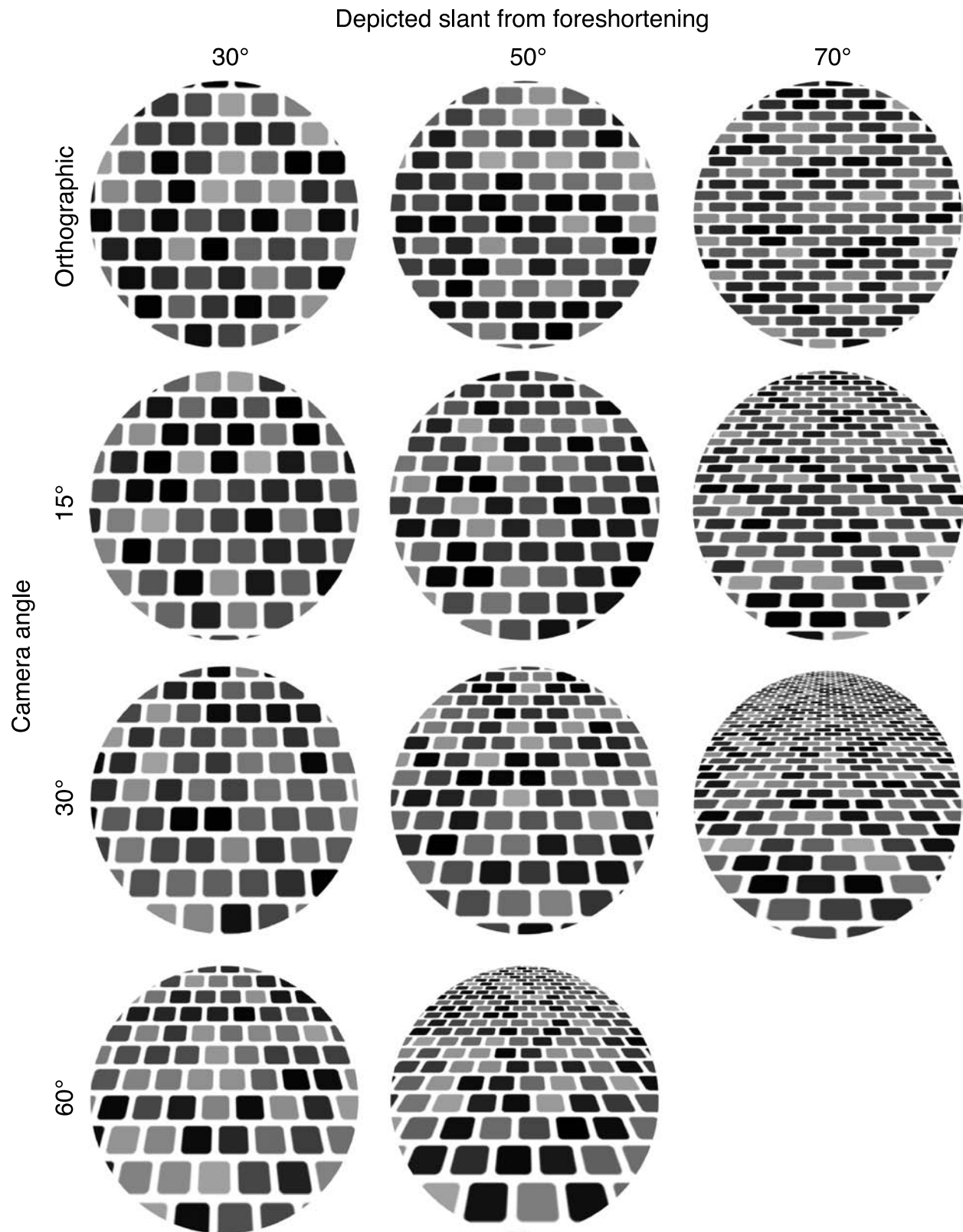
Figure 5. Some sample stimuli from the present series of experiments. The slants of the depicted surfaces were systematically varied, and the images were rendered with a variety of different camera angles. The appearance of slant in these images is enhanced when they are viewed monocularly.
