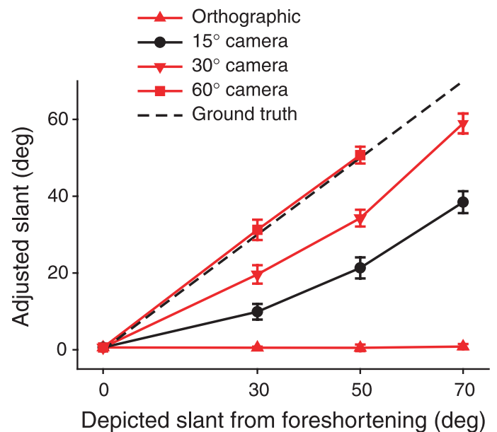
Figure 7. Average judged slants from Experiment 1 as a function of the depicted slant for all of the different camera angles.
