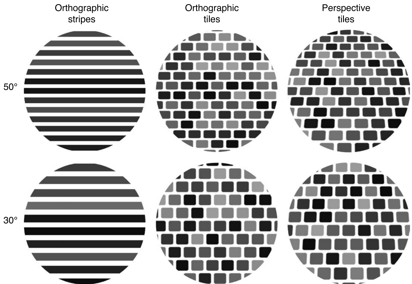
Figure 14. Some sample stimulus pairs from the different conditions of Experiment 5 . All of the differences between the top and bottom rows are well above threshold. Readers should assess whether the differences in apparent slant in the perspective tile images are as salient as the differences in the heights or shapes of their respective texture elements (see also Figure 3 ).
