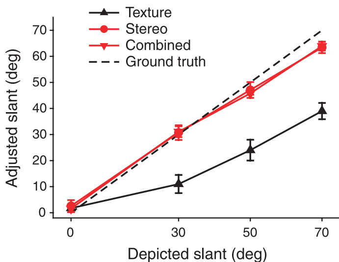
Figure 11. Average judged slants in the stereo-only and cue-consistent conditions from Experiment 3, together with the texture-only data from the same observers in Experiment 1.
