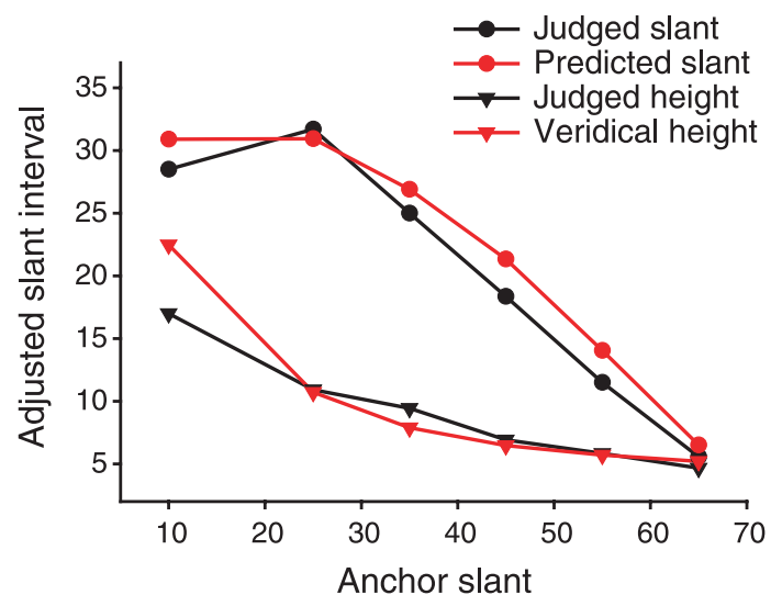
Figure 13. The average settings over all observers in Experiment 4 . The black curves show the adjusted intervals as a function of the anchor slant for each task that appeared equal to the interval between 70^\circ and 75^\circ . The red curves show the predicted performance on the slant task based on scaling contrast and veridical performance on the tile height task.
