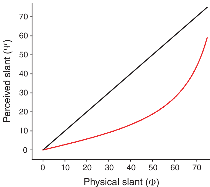
Figure 2. Some hypothetical functions by which perceived slant may be related to the ground truth. The black curve shows the expected pattern of apparent slants for an unbiased observer. The red curve shows the pattern that would be expected based on the scaling contrast model proposed by Todd et al. (2007).
