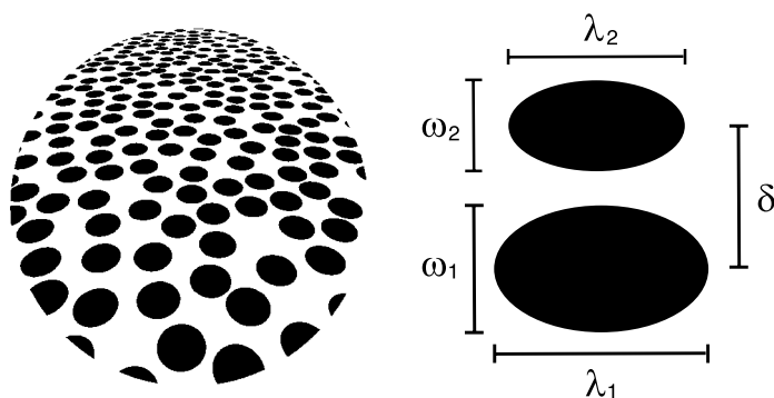
Figure 1. An image of a slanted plane that is perceptually specified by optical texture, and some local measures of texture that are useful for the computation of surface slant.
