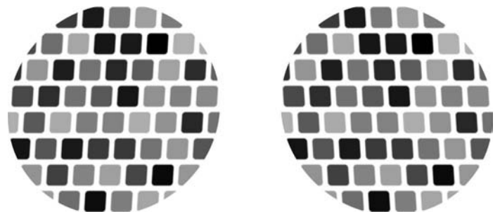
Figure 10. A cue conflict stimulus similar to the ones used in Experiment 3. The pattern of texture in the cyclopean view specifies a frontoparallel surface, whereas the pattern of binocular disparity specifies a surface slanted in depth. In the actual experiment, the tiles were colored in varying shades of red against a black background.
