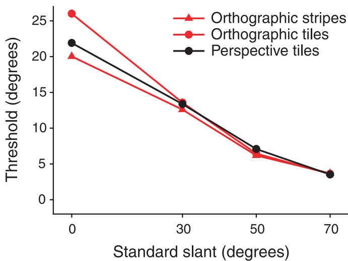
Figure 15. The average thresholds over all observers and staircase directions for the different combinations of texture and perspective used in Experiment 5 .
