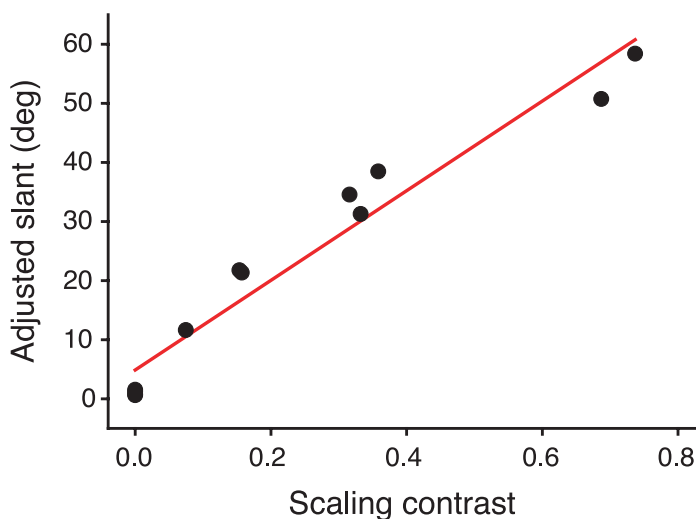
Figure 8. The average judged slants from Experiment 1 as a function of scaling contrast.
