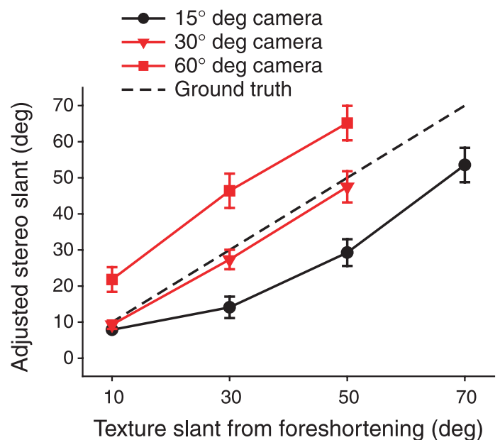
Figure 9. The average judged slants from stereo in Experiment 2 that appeared equal to the apparent slant of a textured surface that was viewed monocularly.
