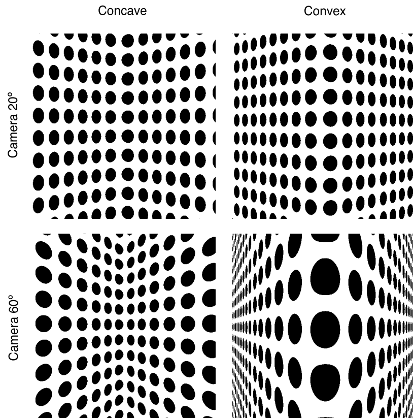
Figure 6. Example images of a concave and a convex surface that were rendered with different camera angles. The asymptotic slant of each depicted surface is 55^\circ .
