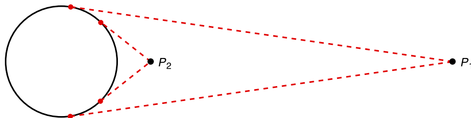
Figure 15. The visible portions of a sphere from two different vantage points P_1 and P_2 . Note how the visible range of depths increases with viewing distance.
