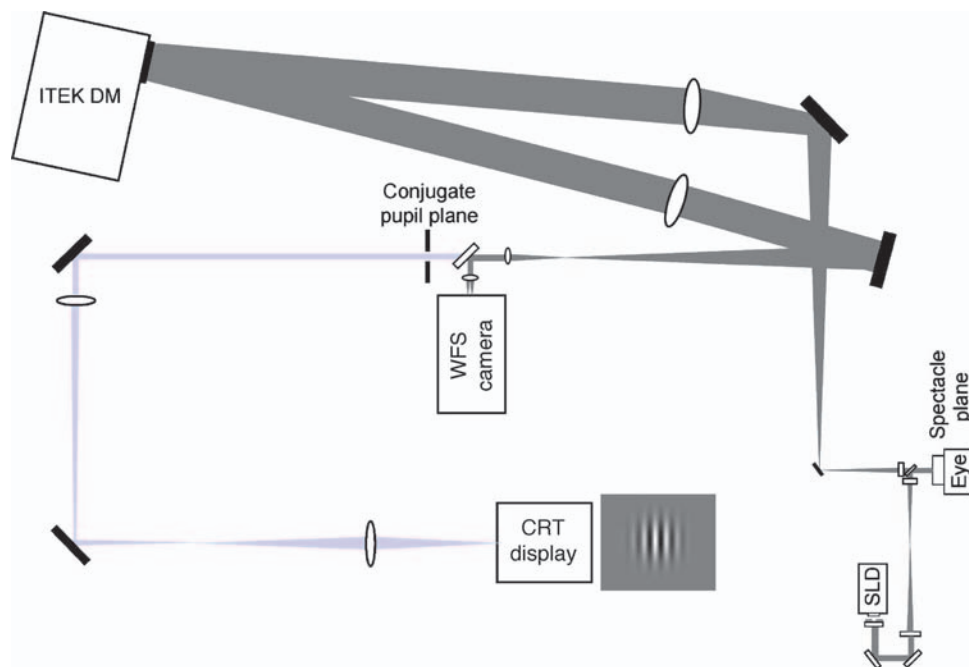
Figure 1. Psychophysics arm of the AO system. Dark gray : AO control loop. Light gray : Non-common CRT light path. The aperture at the conjugate pupil plane was set at either 6 mm or 3 mm depending on the testing condition. Trial lenses were placed in the spectacle plane to correct for 2 nd -order aberrations and an additional trial lens was placed at the conjugate pupil plane to correct for the difference in chromatic focus between the SLD and the CRT display.
