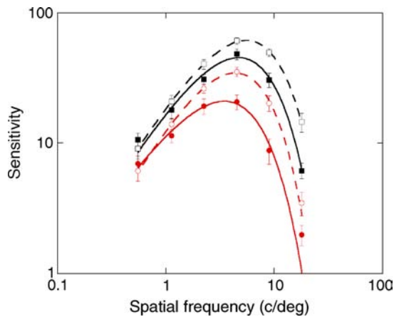
Figure 4. Average contrast sensitivity on a log-log scale for young observers (black symbols and curves) and older observers (red symbols and curves). Solid symbols and curves represent measurements without AO compensation; open symbols and dashed curves denote measurements with AO compensation. Curves were fitted using a double-exponential function. Error bars are \pm 1 SEM.
