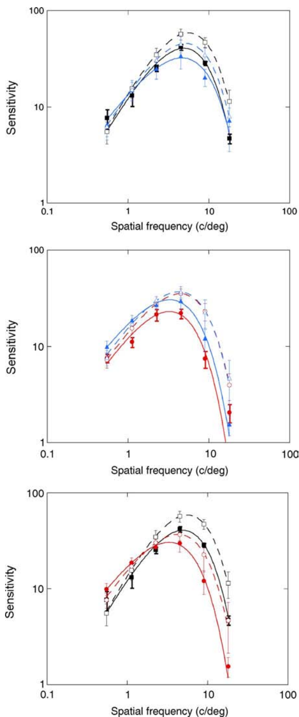
Figure 9. Average contrast sensitivity on a log-log scale compared for the 8 observers used in both the 6 mm and 3 mm pupil conditions. Solid symbols and curves denote measurements without AO compensation; open symbols and dashed curves denote measurements with AO compensation. Top : Younger observer averages. Black symbols and curves signify the 6 mm pupil; blue symbols and curves show the 3 mm pupil. Middle : Older observer averages. Red symbols and curves show the 6 mm pupil average, and blue symbols and curves show the 3 mm pupil. Bottom : Black symbols and curves denote younger observer averages with a 6 mm pupil; red symbols and curves signify older observer averages over a 3 mm pupil.
