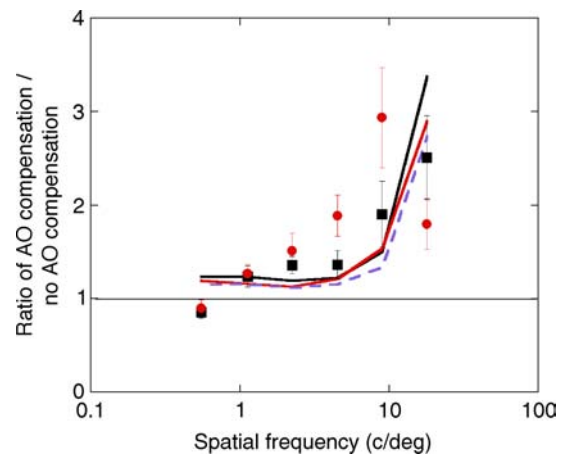
Figure 5. CSF change compared with the TVB of AO compensation for each age group. Solid curves show the TVB, and solid symbols show the CSF change, black and red for young and old, respectively. CSF change is defined as the ratio of contrast sensitivity with AO compensation to that with no AO compensation. TVB is defined as the ratio of degraded retinal image contrast with AO compensation to that with no AO compensation. The dotted blue curve denotes the TVB of older observers with AO compensation relative to young observers with no AO compensation. Error bars are \pm 1 SEM.
