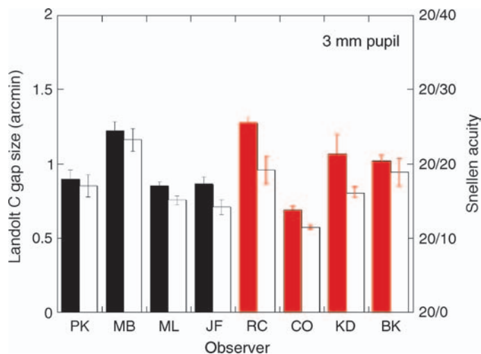
Figure 10. Change in visual acuity with AO compensation for individual observers (black for young, red for older) when measured over a 3 mm pupil, plotted as the minimal resolvable angle in arcmin. Open bars denote visual acuity with AO compensation; solid bars denote visual acuity measured without AO compensation. The right ordinate is Snellen visual acuity. Error bars are \pm 1 SEM.
