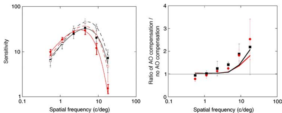
Figure 8. Left : Average contrast sensitivity on a log-log scale for the 3 mm pupil for young (black symbols and curves) and older (red symbols and curves) observers. Solid curves and symbols denote measurements without AO compensation; open symbols and dashed curves denote measurements with AO compensation. Right : The CSF change compared with the TVB of AO compensation for each age group over the 3 mm pupil. Solid curves show the TVB, and solid symbols show the CSF change, black and red for young and old, respectively. Error bars are \pm 1 SEM.
