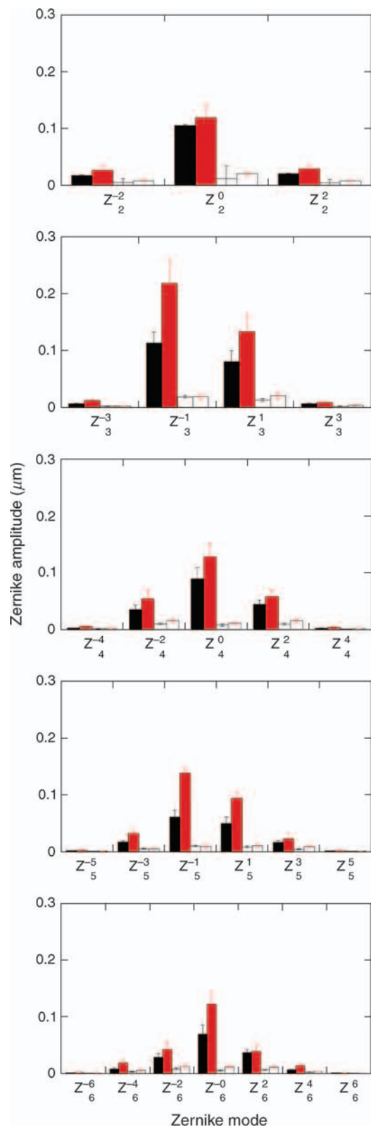
Figure 2. Mean absolute Zernike modes for the younger (black bars), and older (red bars) age groups with (open bars) and without (solid bars) AO compensation over a 6 mm pupil. Each panel represents a separate Zernike radial order. Our DM is capable of correcting aberrations up to the 6 th Zernike radial order. Error bars are \pm 1 SEM.
