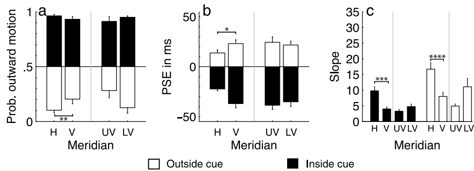
Figure 7. Mean results with distributed cue. (H: horizontal meridian; V: vertical meridian; UV: upper vertical meridian; LV: lower vertical meridian.) Zero Point is higher for outside cue on the vertical meridian, i.e. percept of ILM is weaker than on horizontal meridian (panel a). PSEs and Slopes (panels b and c) show same patterns of significance as single cue (see Figure 5). (Error bars: 1 SE. Significance: * p < .05 ; ** p < .01 ; *** p < .005 ; **** p < .001 .)
