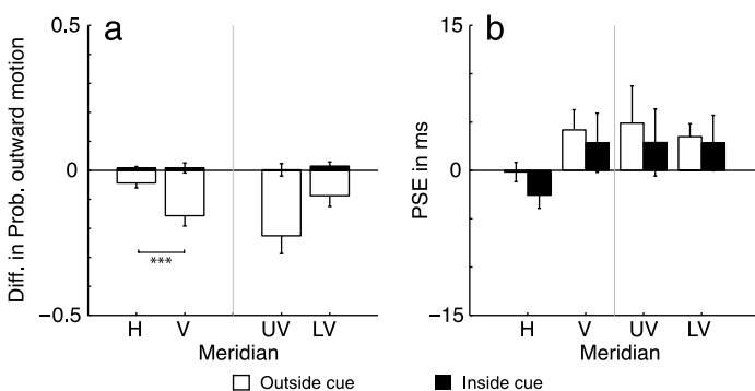
Figure 8. Contribution of attention to ILM is shown as differences between single and distributed cues. (H: horizontal meridian; V: vertical meridian; UV: upper vertical meridian; LV: lower vertical meridian.) (a) Zero Points, and (b) PSEs. ILM is predominantly generated by low-level motion the stimulus in the canonical stimulus configuration. Attention makes a small contribution at the zero points on the vertical meridian, which is significantly greater than on the horizontal meridian. (Error bars: 1 SE. Significance: * p < .05 ; ** p < .01 ; *** p < .005 ; **** p < .001 .)
