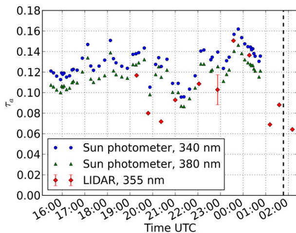
FIG. 2. Time series of lidar AOT at 355 nm and sun photometer AOT at 340 and 380 nm taken at 26 Feb 2013 in El Segundo; sunset at 0147 UTC (dashed line).
