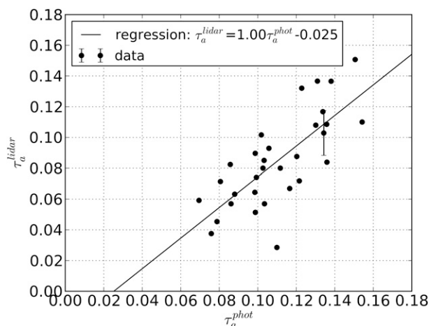
FIG. 3. Scatterplot of lidar AOT vs time-coincident sun photometer AOT at 355 nm for the campaign from 13 to 28 Feb 2013 in El Segundo; R^2 = 0.55 .
