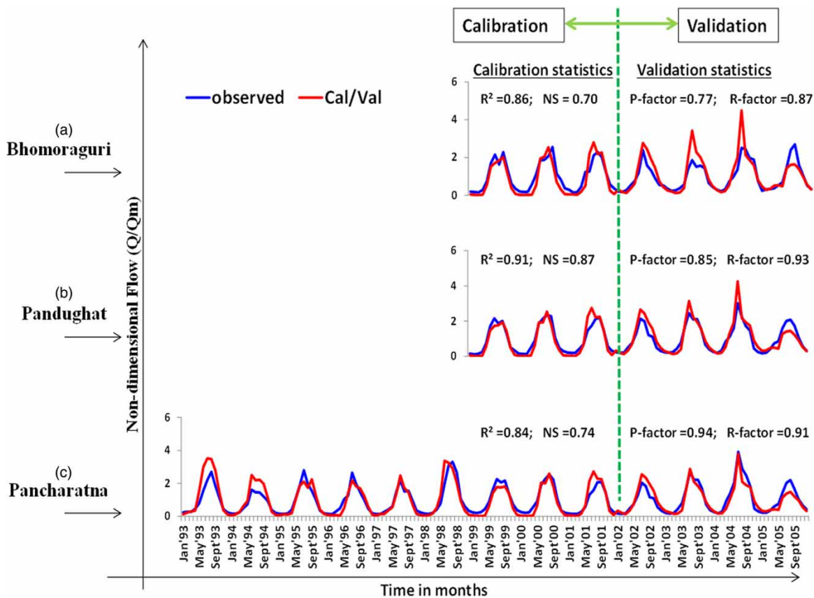
Figure 6 | Results of multi-outlet calibration and validation results of MODEL_6. The calibration and validation results of the monthly model are plotted in a single plot showing the non-dimensional flow ( Q/Q_m ) values. Here, Q represents flow (simulated or observed) and Q_m represents the mean of five-year flow data selected on a random basis.
