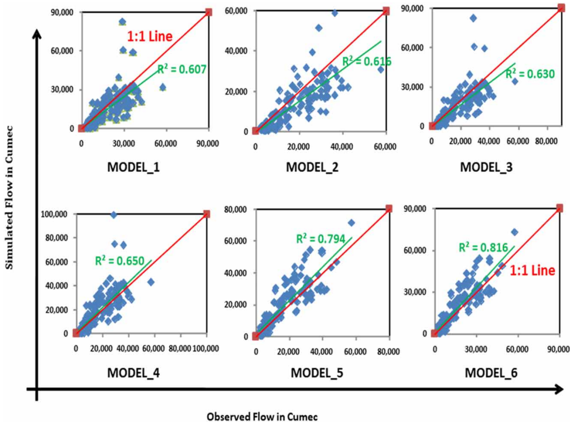
Figure 4 | Scatter plot of monthly simulated flows ( \text{m}^3/\text{s} ) against the corresponding measured discharges ( \text{m}^3/\text{s} ) at Pancharatna for all SWAT models. Here, simulated values indicate the monthly outputs obtained from model run (1991–2012, for the first four models and 1991–2005, for the last two models) without calibration and validation.
