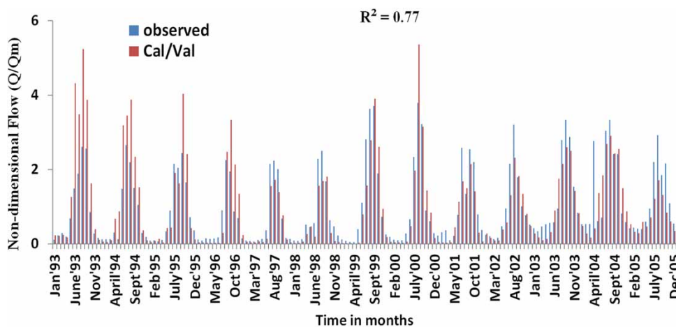
Figure 7 | Performance of MODEL_6 at tributary basin. This plot shows the comparison of non-dimensional flows ( Q/Q_m ) between the outputs of model final run and the observed values at Golaghat outlet in Dhansiri river basin. Here, Q represents flow (simulated or observed) and Q_m represents the mean of five-year flow data selected on a random basis.
