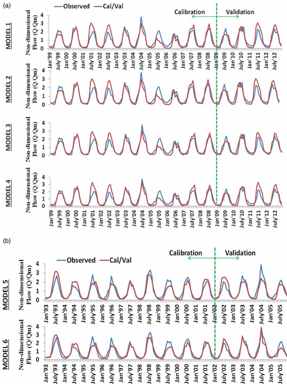
Figure 5 | (a) Results of single-outlet calibration (1999–2008) and validation (2009–2012) at Pancharatna of the first four SWAT models (i.e., MODEL_1, MODEL_2, MODEL_3, MODEL_4). The calibration and validation results of the monthly models are plotted in a single plot showing the non-dimensional flow ( Q/Q_m ) values. Here, Q represents flow (simulated or observed) and Q_m represents the mean of five-year flow data selected on a random basis. (b) Results of single-outlet calibration (1993–2001) and validation (2002–2005) at Pancharatna of the last two SWAT models (i.e., MODEL_5 and MODEL_6). The calibration and validation results of the monthly models are plotted in a single plot showing the non-dimensional flow ( Q/Q_m ) values. Here, Q represents flow (simulated or observed) and Q_m represents the mean of five-year flow data selected on a random basis.
