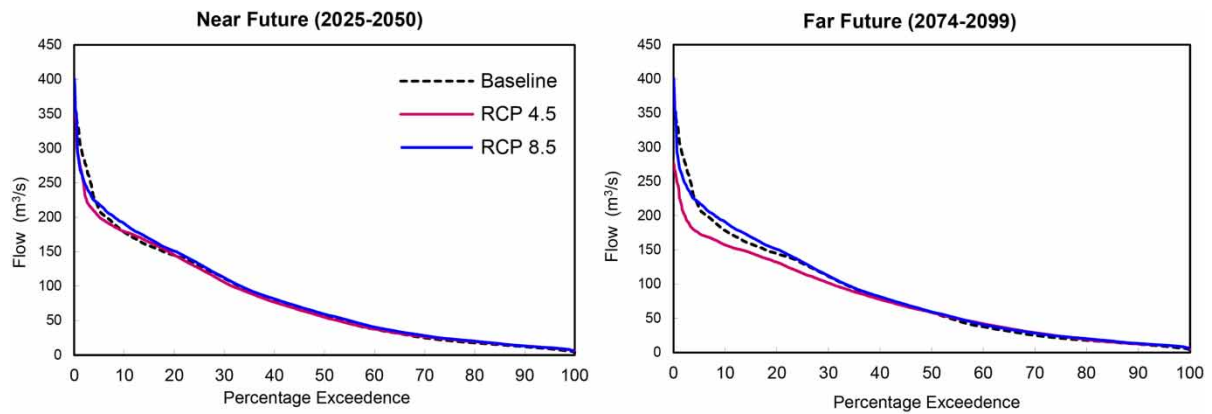
Figure 6 | Comparison of flow duration curve at the outlet during under baseline, RCP 4.5 and RCP 8.5 in near (2025–2050) and far future (2074–2099) in the study basin.
