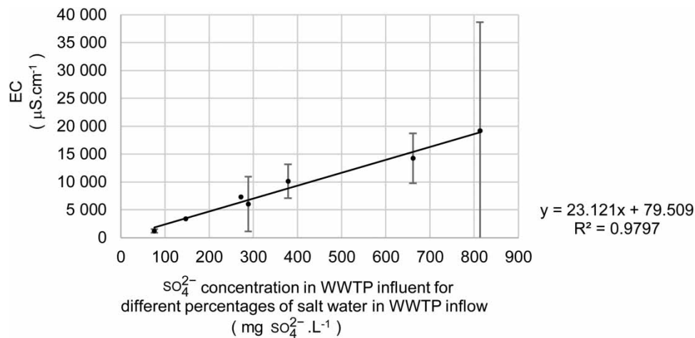
Figure 9 | Correlation between EC and SO 4 2- concentration in WWTP influent.
