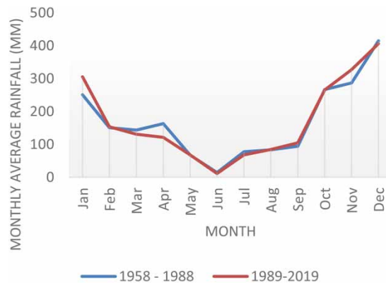
Figure 7 | First 30 years to second 30 years' annual rainfall pattern variation in Zone 1 (1958–2019).
