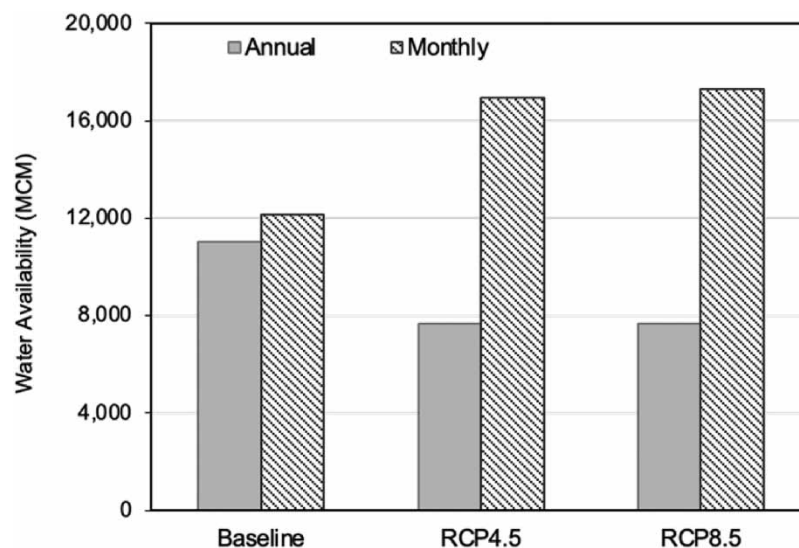
Figure 3 | The average annual and monthly water availability (MCM: million cubic metres) in Kaski District, Nepal, for a future period (2022–2050) under RCP4.5 and RCP8.5 emission scenarios compared with baseline (1992–2010).
