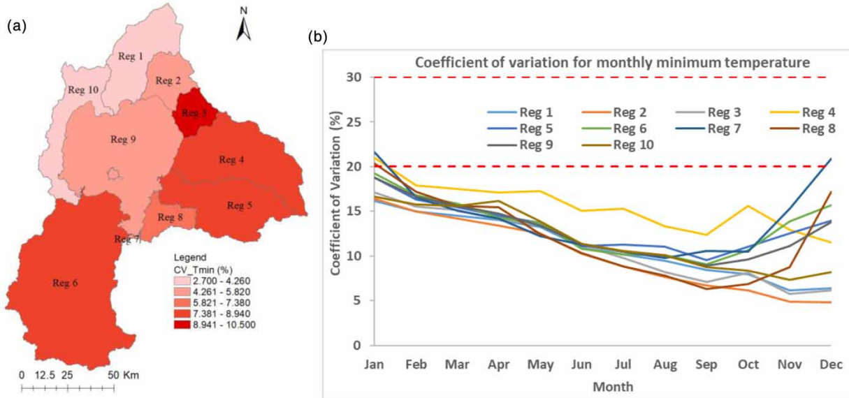
Figure 4 | CV for (a) annual and (b) monthly minimum temperature.
