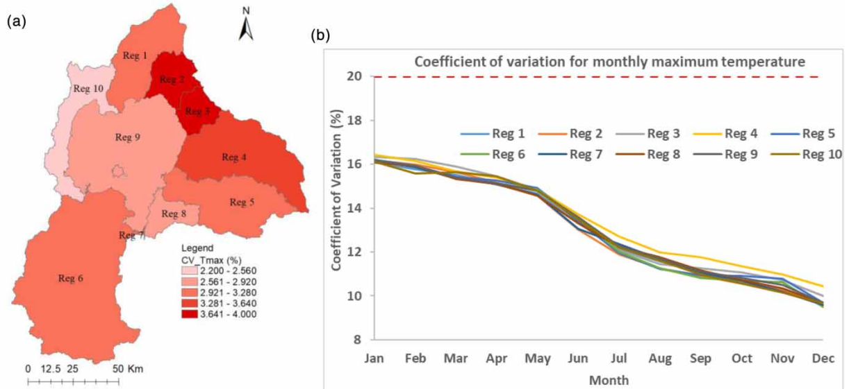
Figure 5 | CV for (a) annual and (b) monthly maximum temperature.
