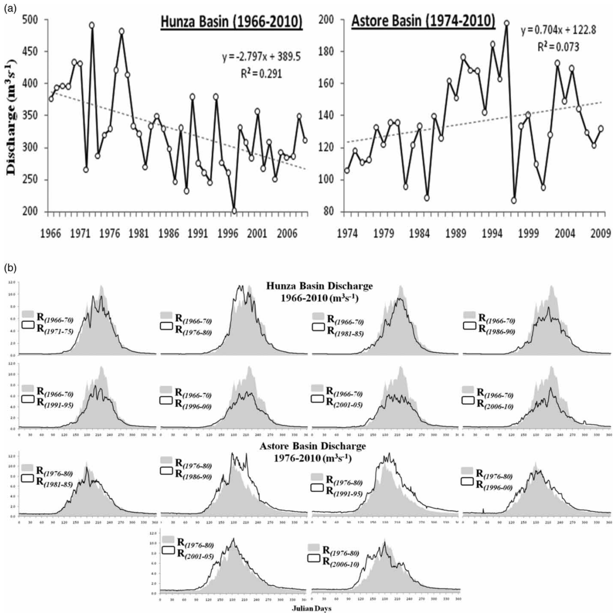
Figure 5 | (a) Annual discharge trends; and (b) Pentad five-year daily mean discharge fluctuations from the base period for the Hunza and Astore basins.
