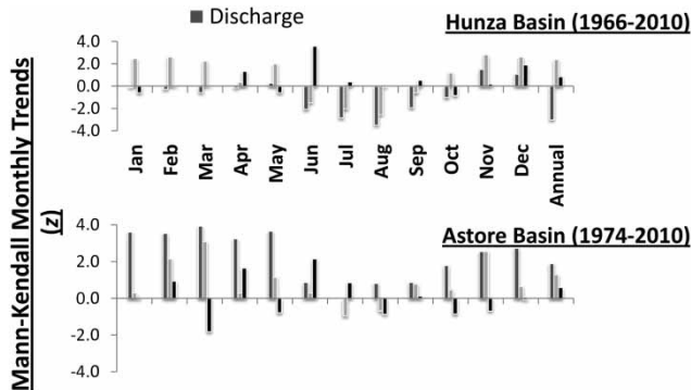
Figure 4 | Temperature, precipitation and discharge trends for the Astore and Hunza basins; values \geq 1.96 and \leq -1.96 represents a trend significance level \alpha < 0.01 .
