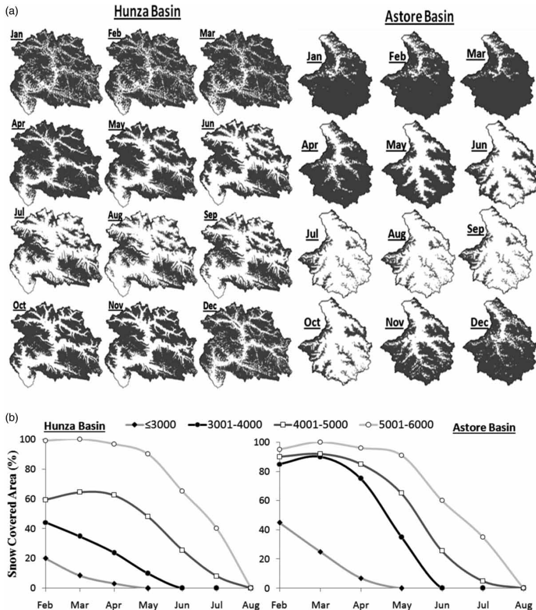
Figure 3 | (a) Extent of mean monthly basin snow cover; (b) Mean monthly snow cover recession curves.
