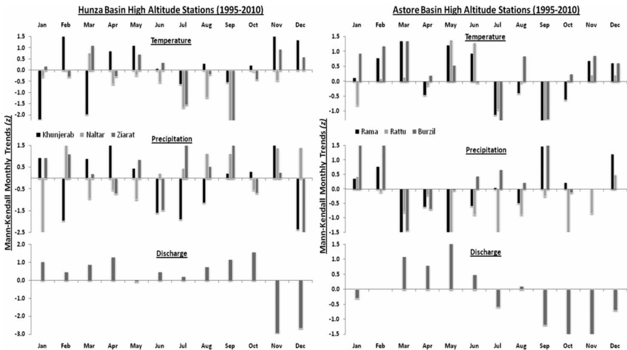
Figure 6 | Monthly temperature, precipitation and discharge trends during 1995–2010 for the Hunza and Astore basin high altitude stations; values \geq 1.96 and \leq -1.96 represent a trend significance level \alpha < 0.01 .
