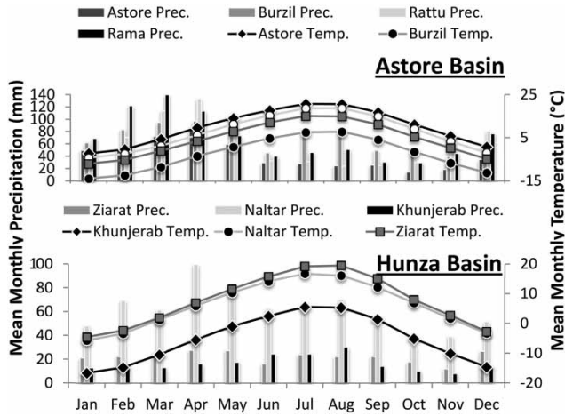
Figure 2 | Mean monthly temperature and precipitation for the Astore and Hunza basins.
