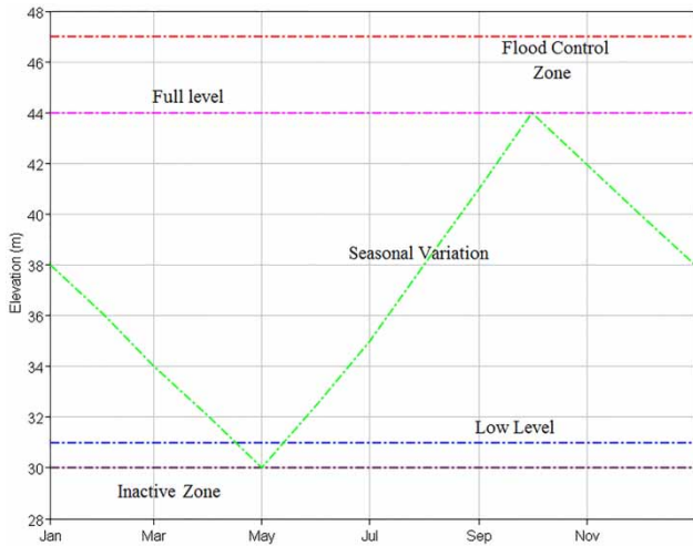
Figure 3 | Annual operation rules for Stung Sen dam.
