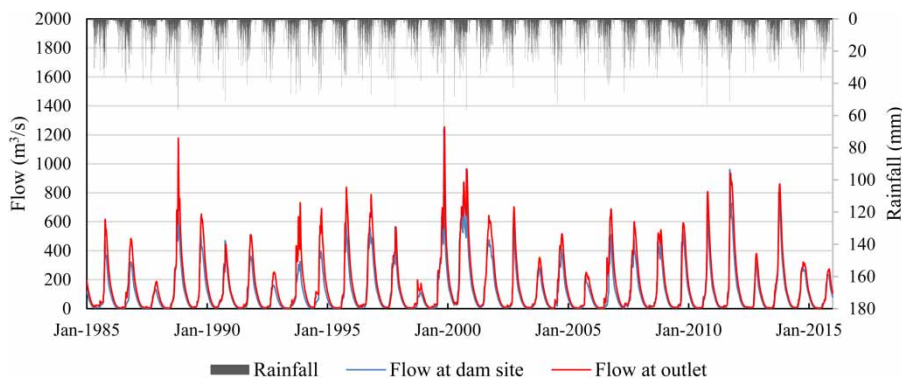
Figure 5 | Simulated daily hydrograph at both the outlet and proposed dam site (1985–2015).
