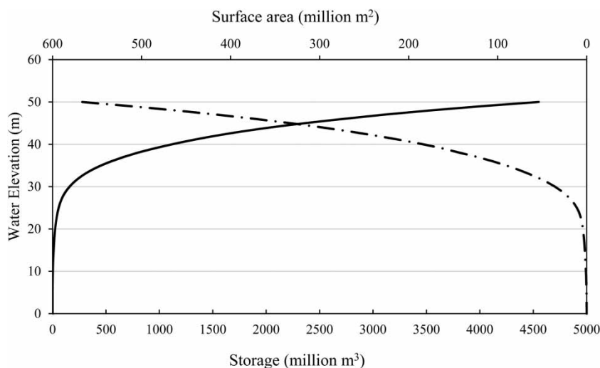
Figure 2 | Elevation–volume–area curve of Stung Sen dam reservoir.
