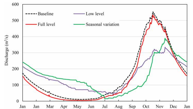
Figure 9 | Average flow at the outlet of Stung Sen Basin under different operation rules.
