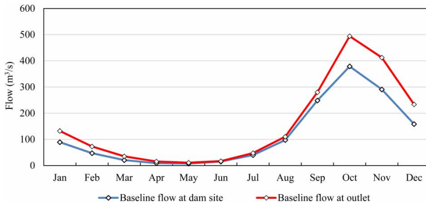
Figure 6 | Average simulated monthly hydrograph at both outlet and proposed dam site.
