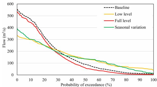
Figure 8 | Flow duration curves at the outlet of Stung Sen Basin under different operation rules.
