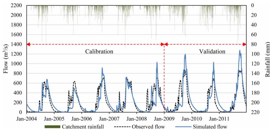
Figure 4 | Comparison of simulated and observed daily hydrograph at the outlet for both calibration and validation periods.
