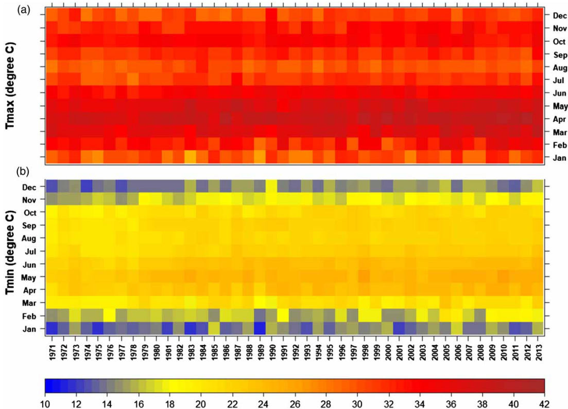
Figure 2 | Temporal distributions of temperature variables over the KYB: (a) maximum temperature ( ^{\circ}\text{C} ), (b) minimum temperature ( ^{\circ}\text{C} ).
