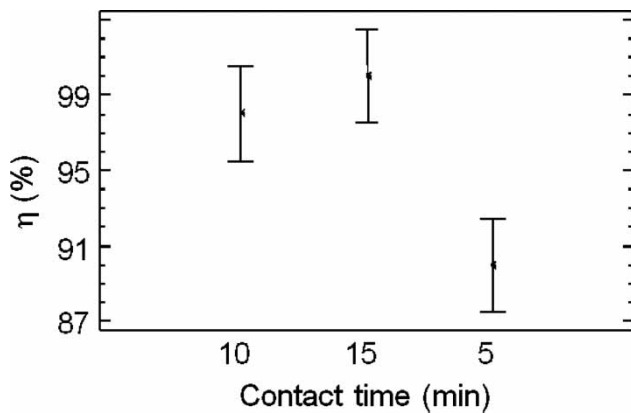
Figure 2 | PAA disinfection efficiency as a function of contact time in continuous flow experiments, for a constant concentration of 15 mg/L, 95.0% confidence interval.
