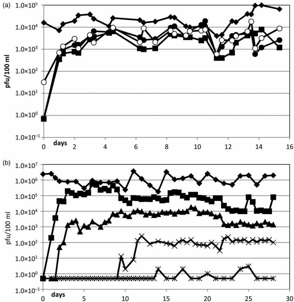
Figure 2 | Phage removal after 1 m infiltration distance in columns run at different PWVs; symbols in (a) (○) 4; (●) 2; (■) 1 m/d. Symbols in (b) (■) 1; (▲) 0.5; (×) 0.25; (∗) 0.1 m/d. In (a) and (b) the input symbol is (◆).
